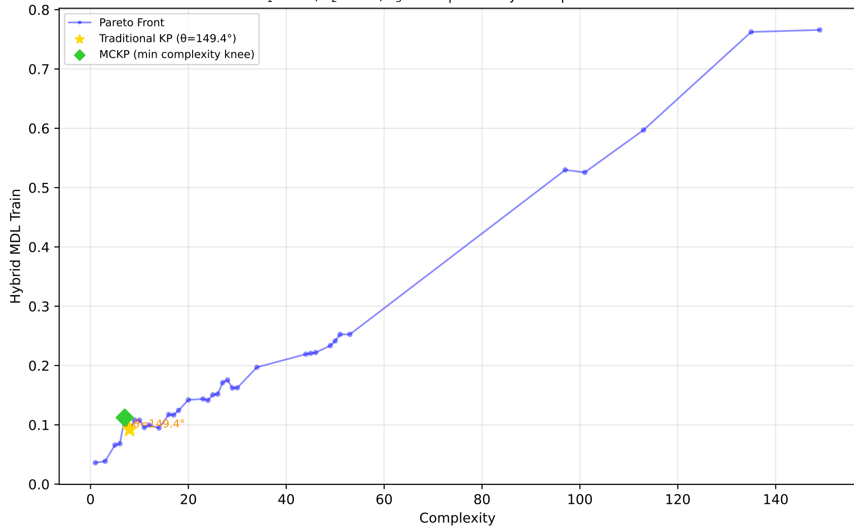
522_pm10 - Run 14 - SVP - Hybrid MDL Train \lambda_1=1.00, \lambda_2=0.00, \lambda_3=0.90 | Difficulty: 1.00 | Method: hmr
