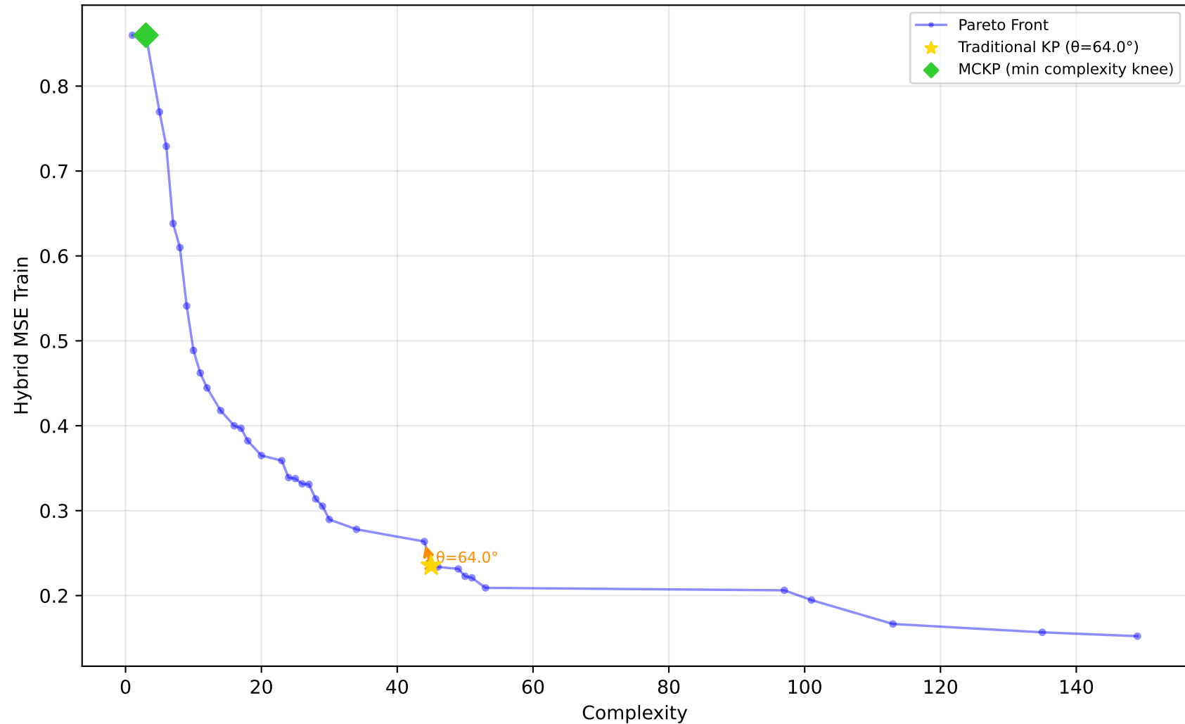
522_pm10 - Run 14 - SVP - Hybrid MSE Train \lambda_1=0.00, \lambda_2=0.10, \lambda_3=0.00 | Difficulty: 1.00 | Method: hmr
