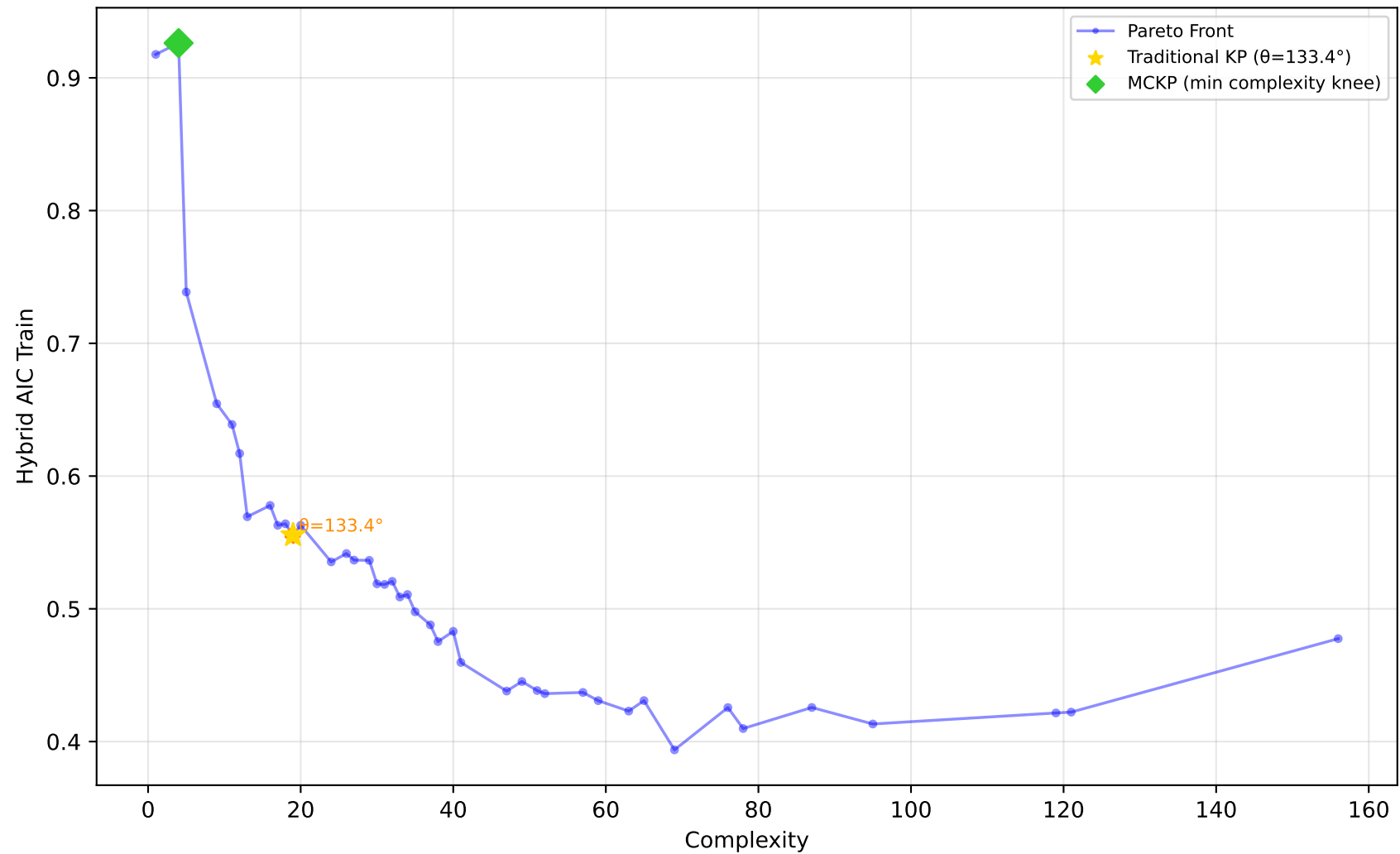
522_pm10 - Run 15 - MVP - Hybrid AIC Train \lambda_1=0.00, \lambda_2=0.90, \lambda_3=0.00 | Difficulty: 1.00 | Method: hmr
