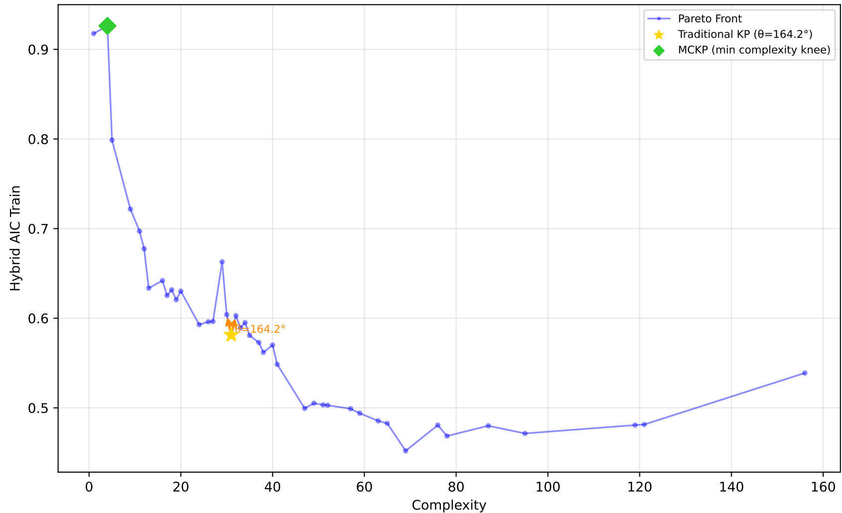
522_pm10 - Run 15 - MVP - Hybrid AIC Train \lambda_1=1.00, \lambda_2=0.00, \lambda_3=0.00 | Difficulty: 1.00 | Method: hmr
