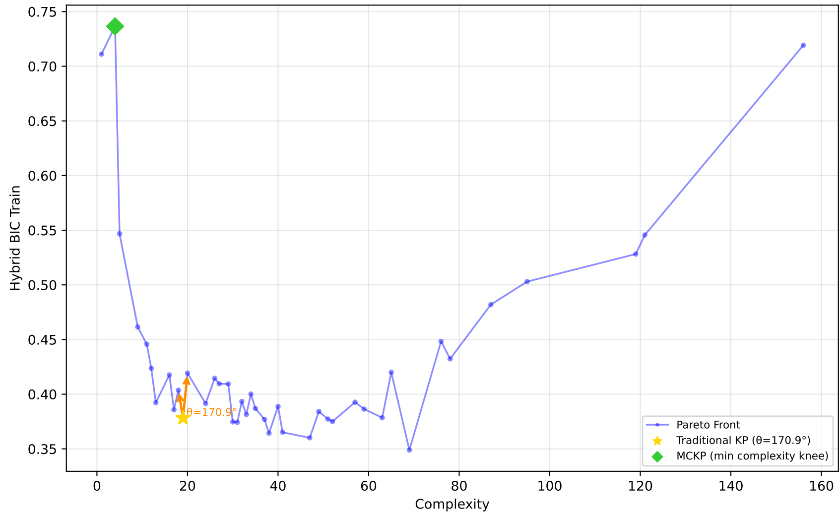
522_pm10 - Run 15 - MVP - Hybrid BIC Train \lambda_1=0.00, \lambda_2=0.90, \lambda_3=0.00 | Difficulty: 1.00 | Method: hmr
