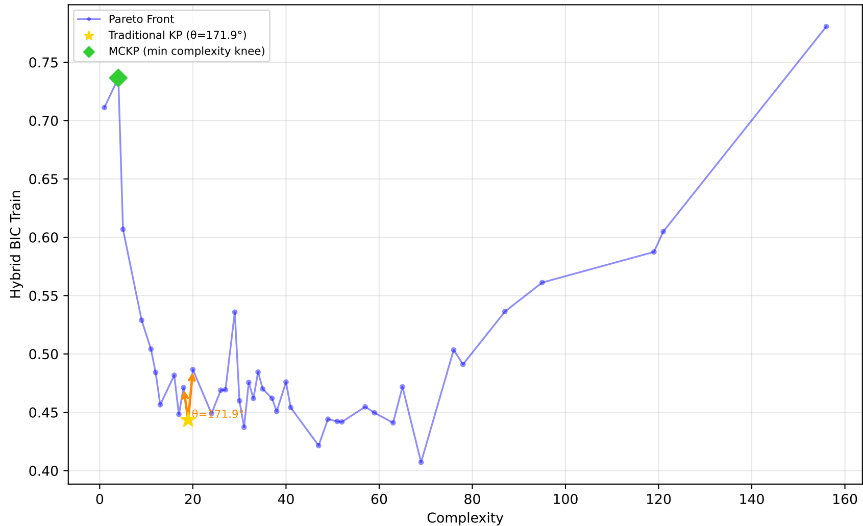
522_pm10 - Run 15 - MVP - Hybrid BIC Train \lambda_1=1.00, \lambda_2=0.00, \lambda_3=0.00 | Difficulty: 1.00 | Method: hmr
