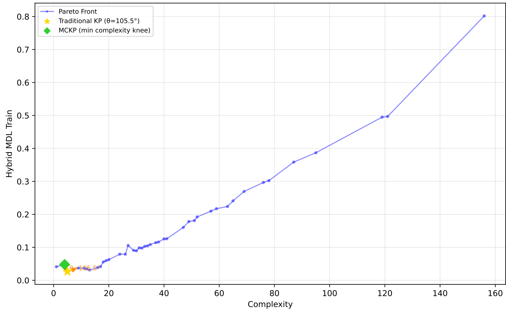
522_pm10 - Run 15 - MVP - Hybrid MDL Train \lambda_1=0.00, \lambda_2=0.90, \lambda_3=0.00 | Difficulty: 1.00 | Method: hmr
