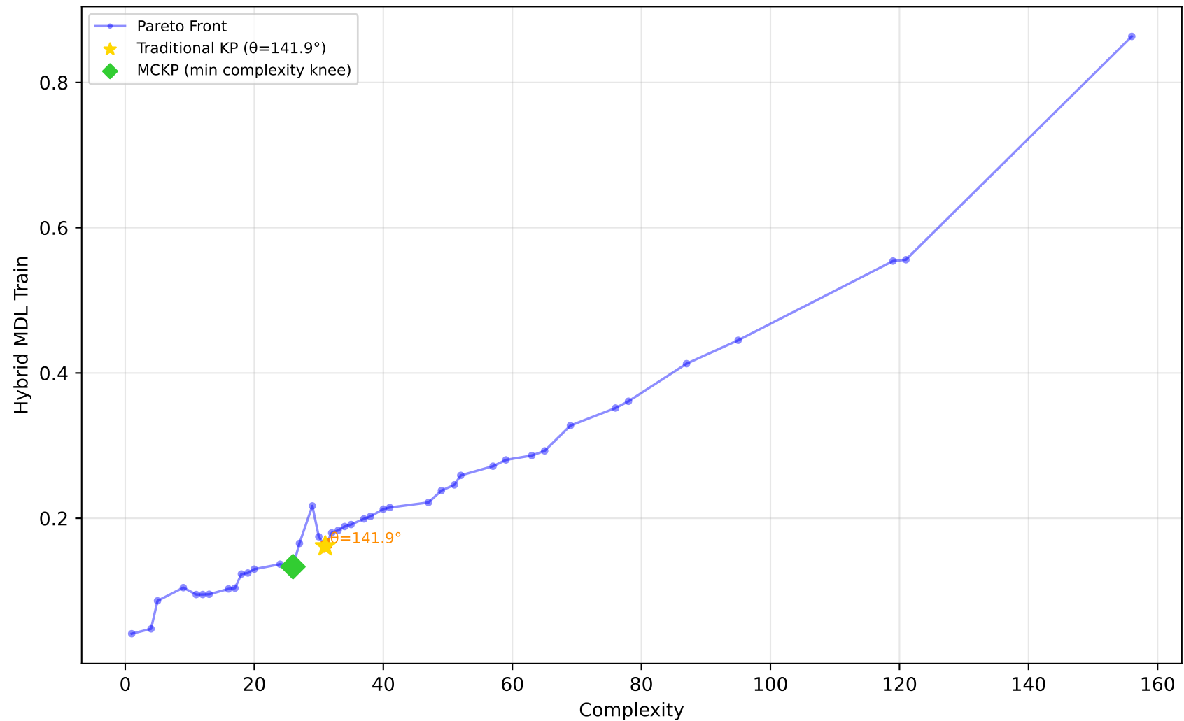
522_pm10 - Run 15 - MVP - Hybrid MDL Train \lambda_1=1.00, \lambda_2=0.00, \lambda_3=0.00 | Difficulty: 1.00 | Method: hmr
