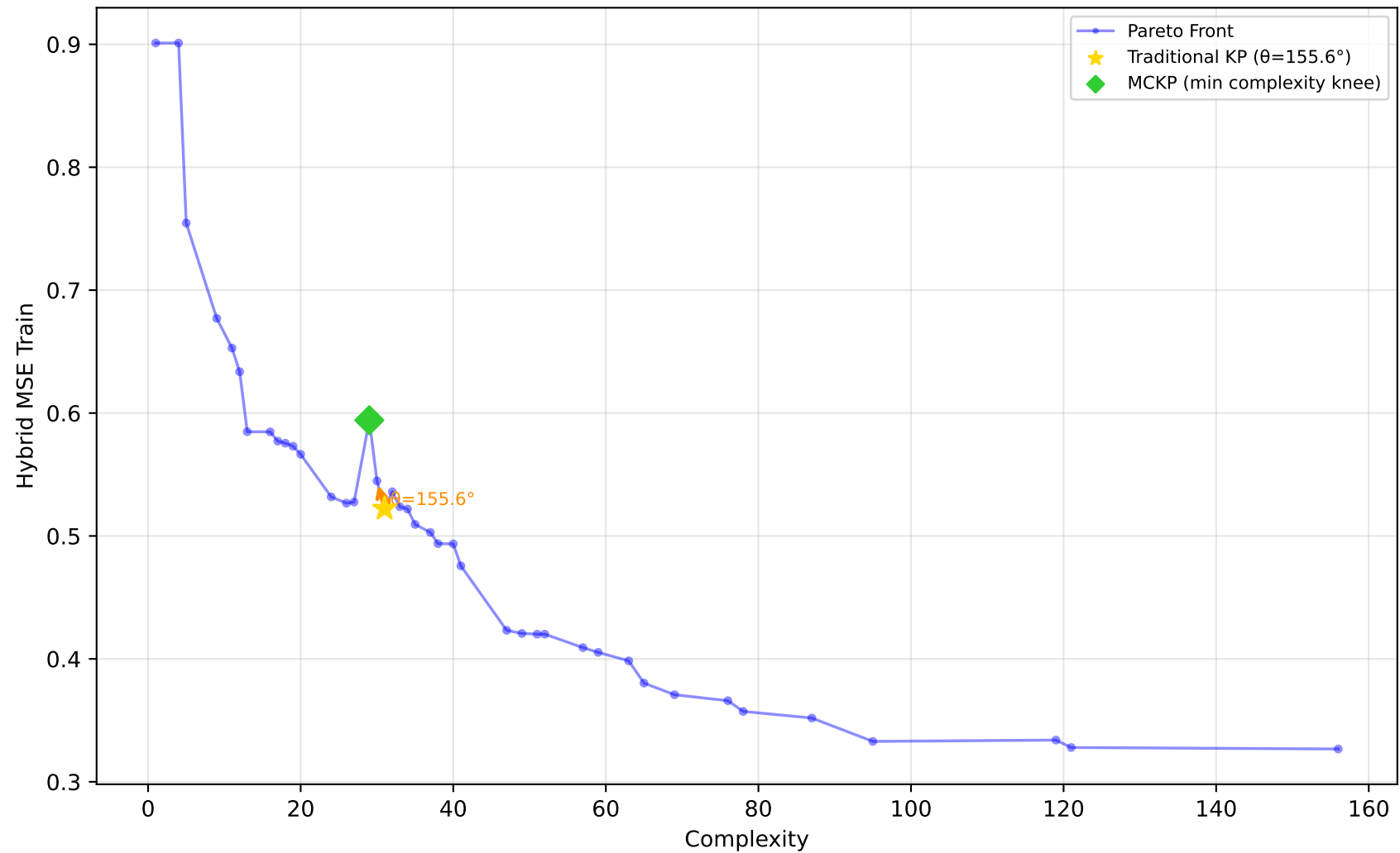
522_pm10 - Run 15 - MVP - Hybrid MSE Train \lambda_1=1.00, \lambda_2=0.00, \lambda_3=0.00 | Difficulty: 1.00 | Method: hmr
