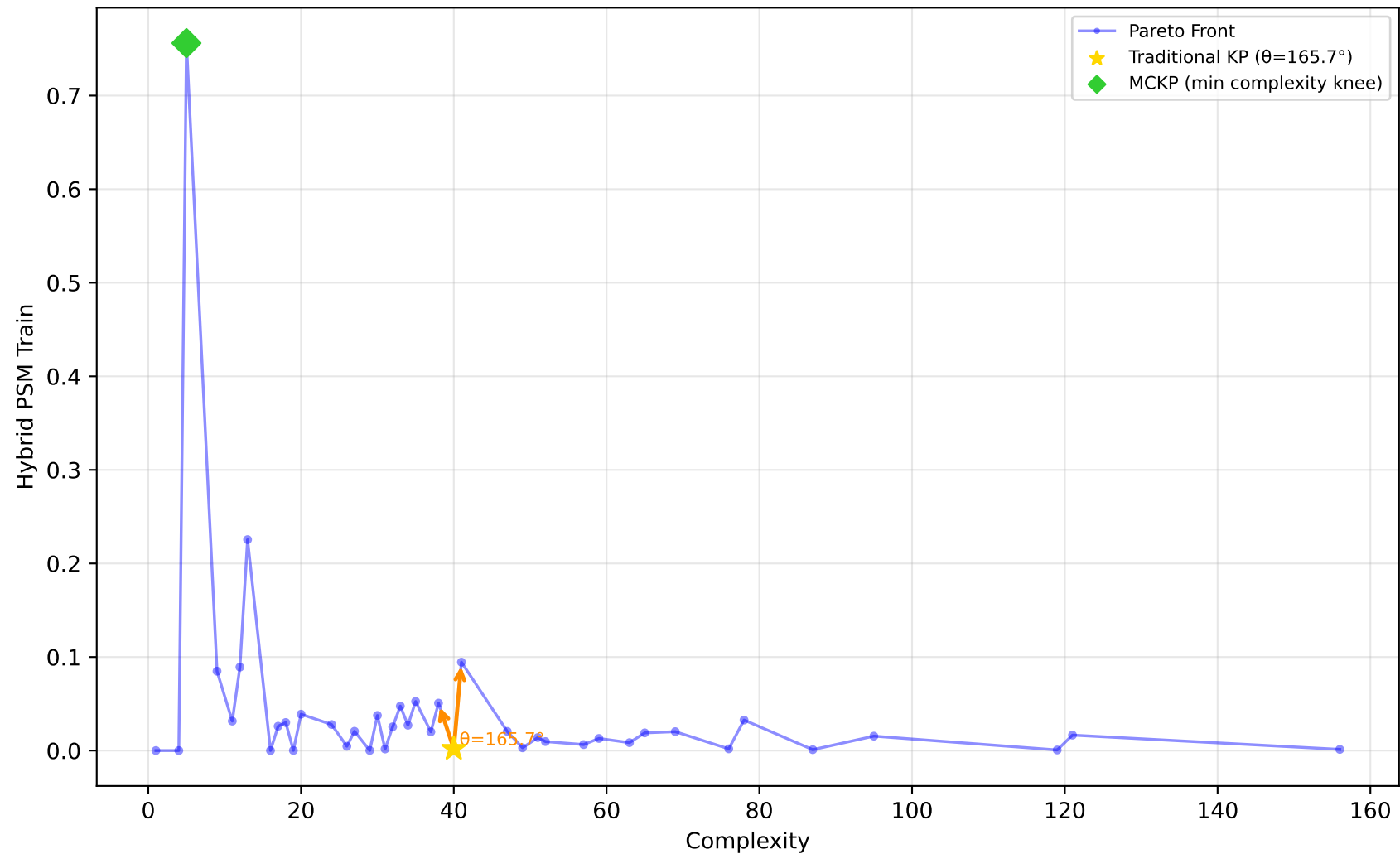
522_pm10 - Run 15 - MVP - Hybrid PSM Train \lambda_1=0.00, \lambda_2=0.90, \lambda_3=0.00 | Difficulty: 1.00 | Method: hmr
