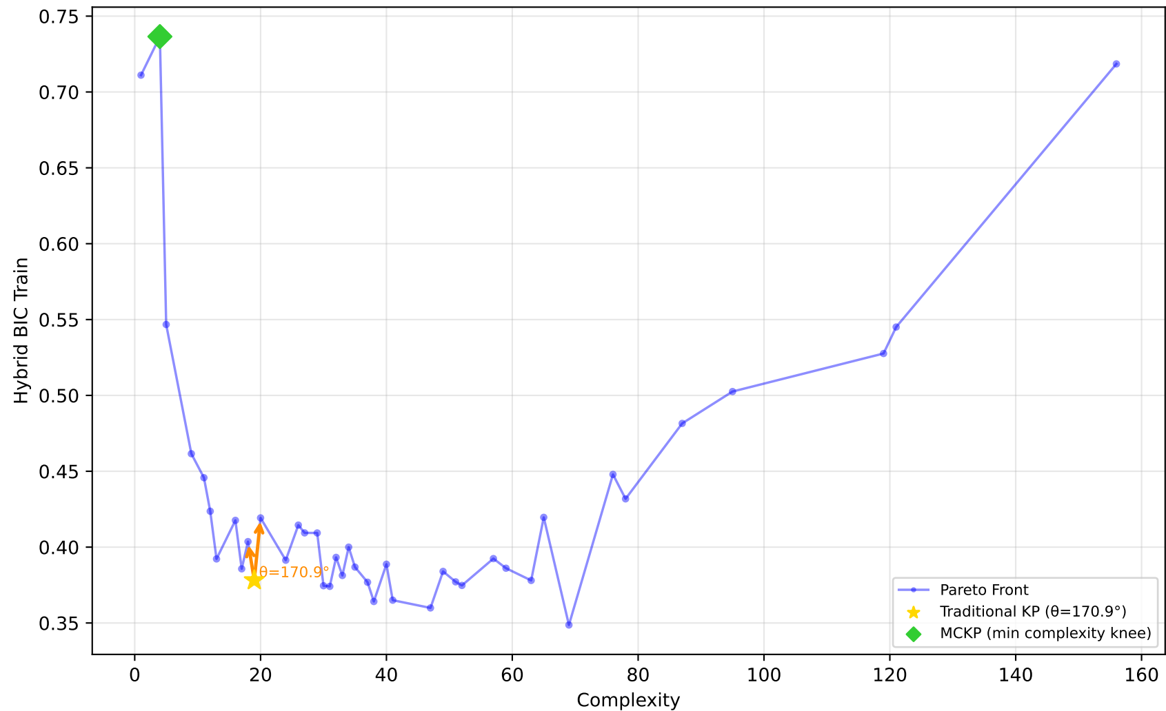
522_pm10 - Run 15 - SVP - Hybrid BIC Train \lambda_1=0.00, \lambda_2=0.10, \lambda_3=0.00 | Difficulty: 1.00 | Method: hmr
