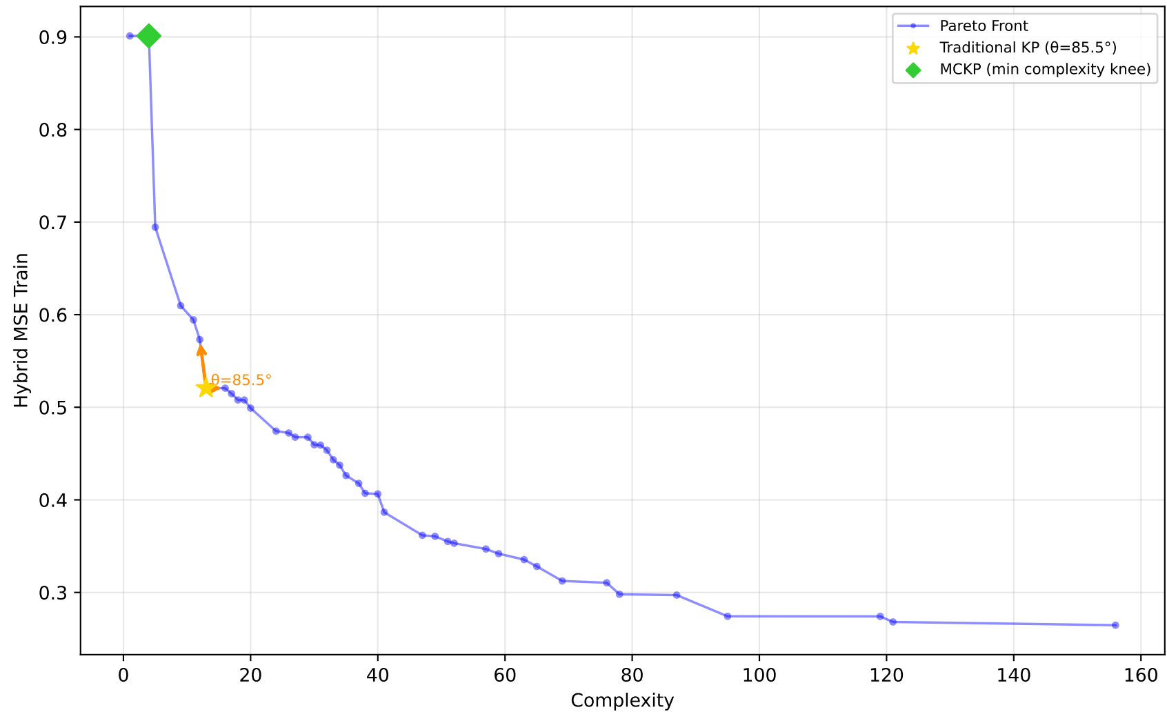
522_pm10 - Run 15 - SVP - Hybrid MSE Train \lambda_1=0.00, \lambda_2=0.10, \lambda_3=0.00 | Difficulty: 1.00 | Method: hmr
