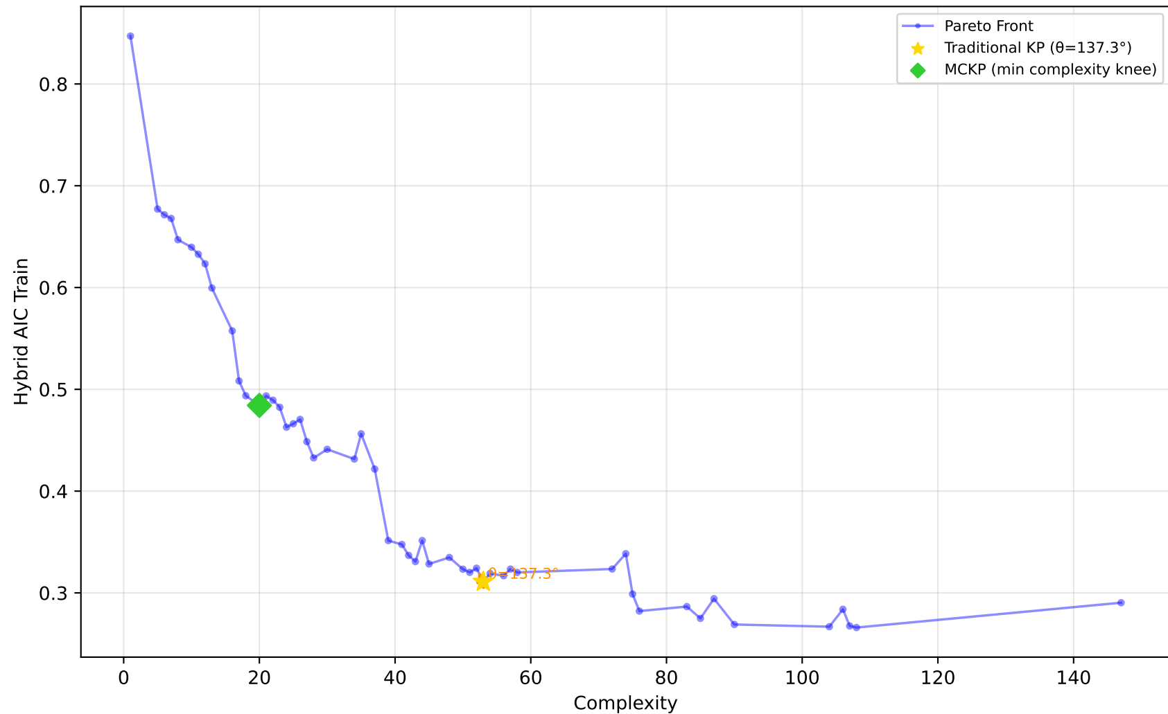
522_pm10 - Run 16 - MVP - Hybrid AIC Train \lambda_1=1.00, \lambda_2=0.00, \lambda_3=0.00 | Difficulty: 1.00 | Method: hmr
