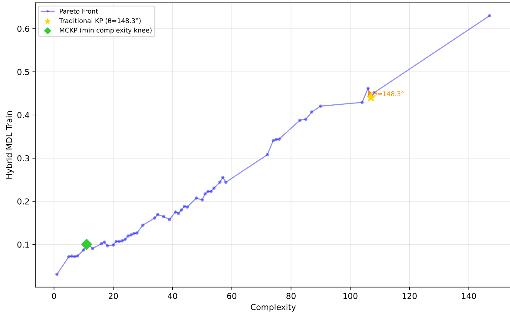
522_pm10 - Run 16 - MVP - Hybrid MDL Train \lambda_1=1.00, \lambda_2=0.00, \lambda_3=0.00 | Difficulty: 1.00 | Method: hmr
