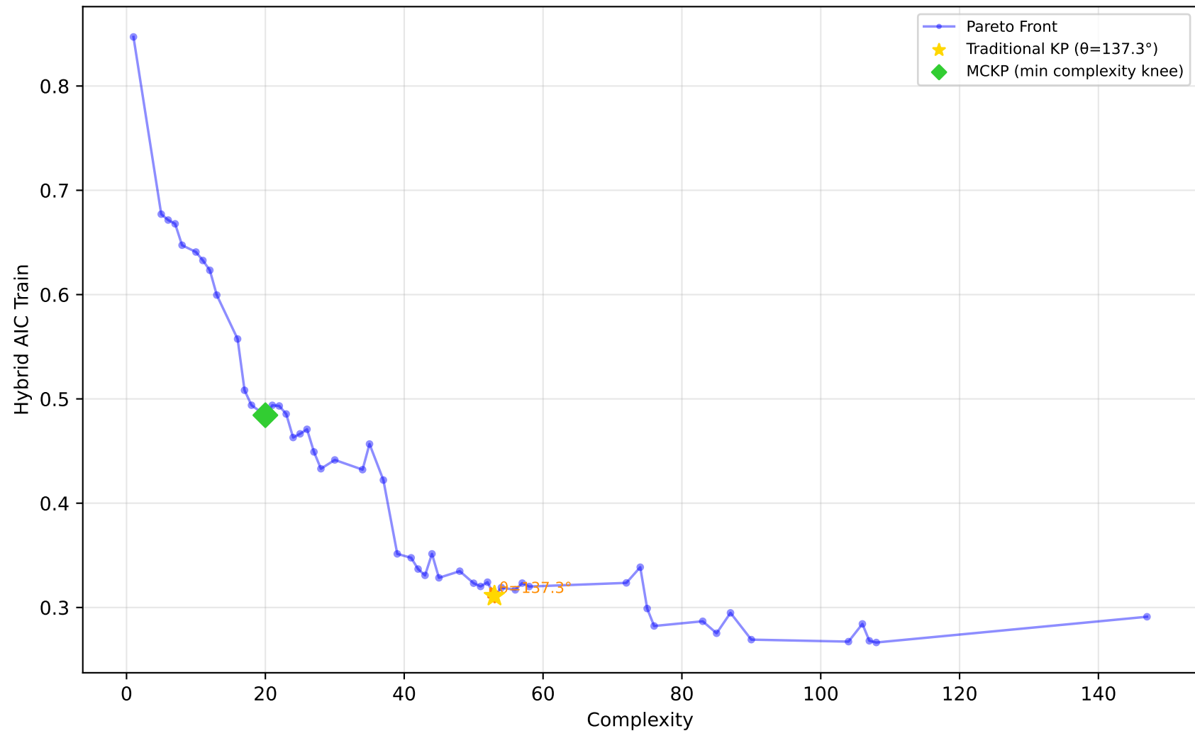
522_pm10 - Run 16 - SVP - Hybrid AIC Train \lambda_1=1.00, \lambda_2=0.00, \lambda_3=0.90 | Difficulty: 1.00 | Method: hmr
