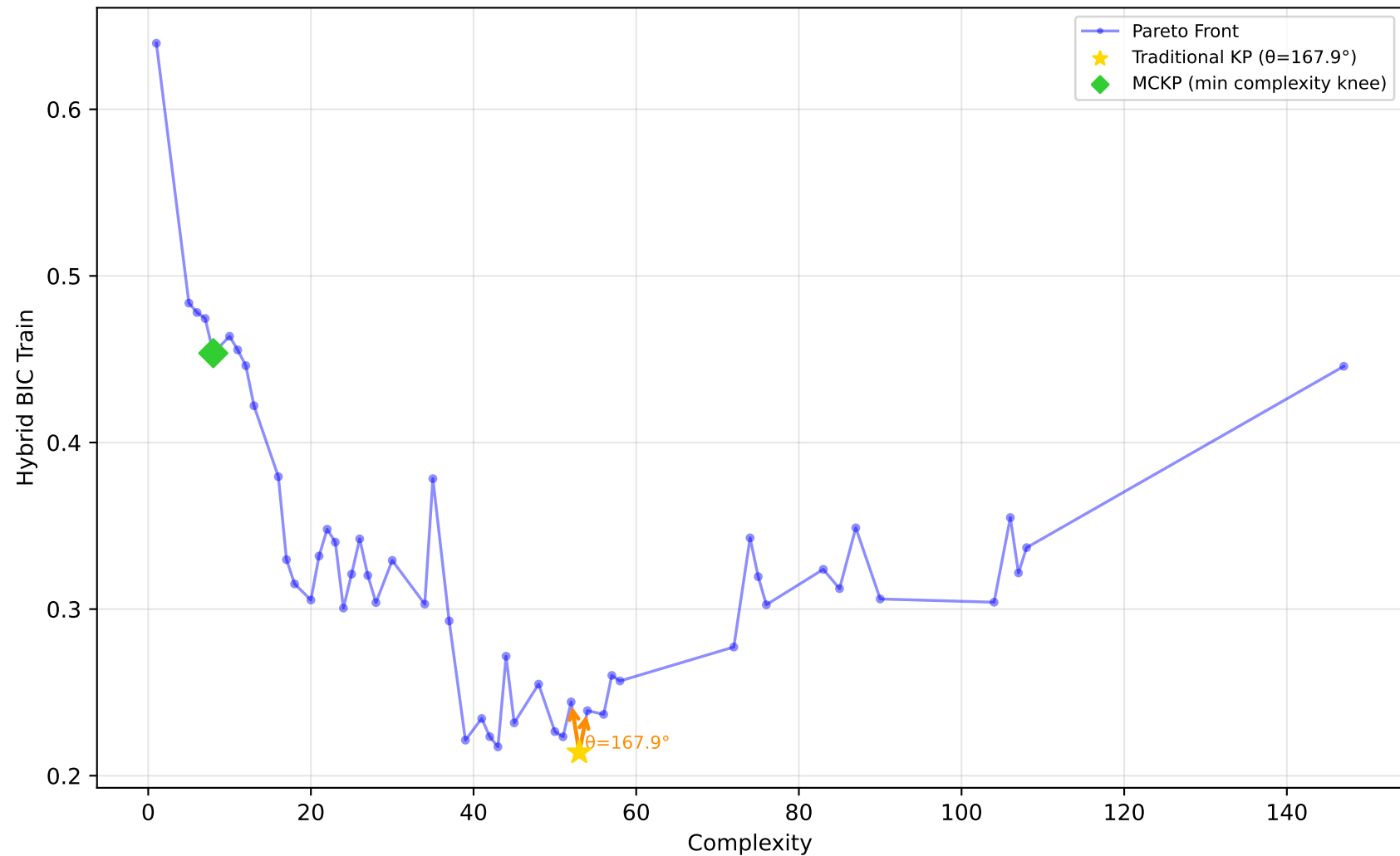
522_pm10 - Run 16 - SVP - Hybrid BIC Train \lambda_1=1.00, \lambda_2=0.00, \lambda_3=0.90 | Difficulty: 1.00 | Method: hmr
