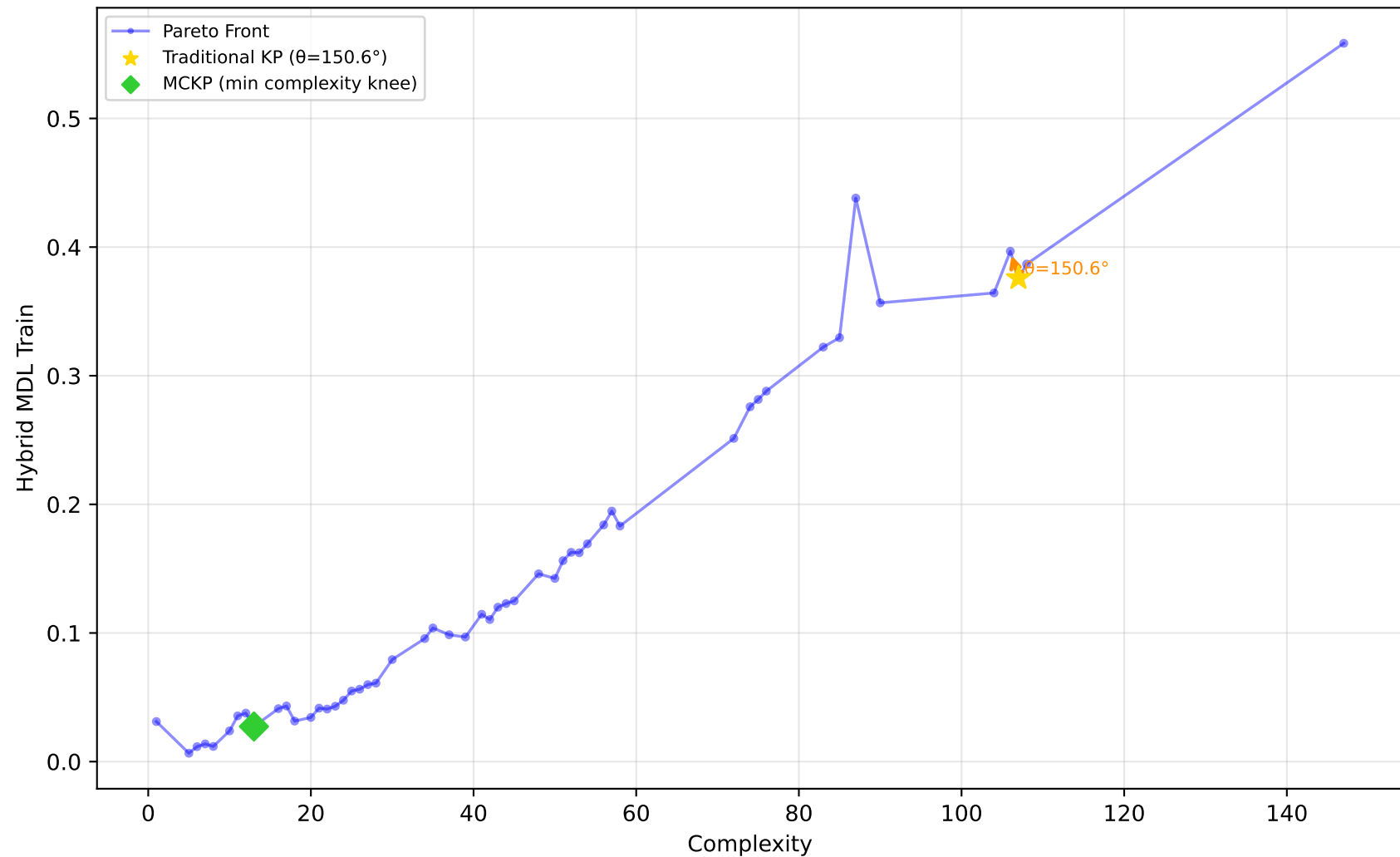
522_pm10 - Run 16 - SVP - Hybrid MDL Train \lambda_1=0.00, \lambda_2=0.10, \lambda_3=0.00 | Difficulty: 1.00 | Method: hmr
