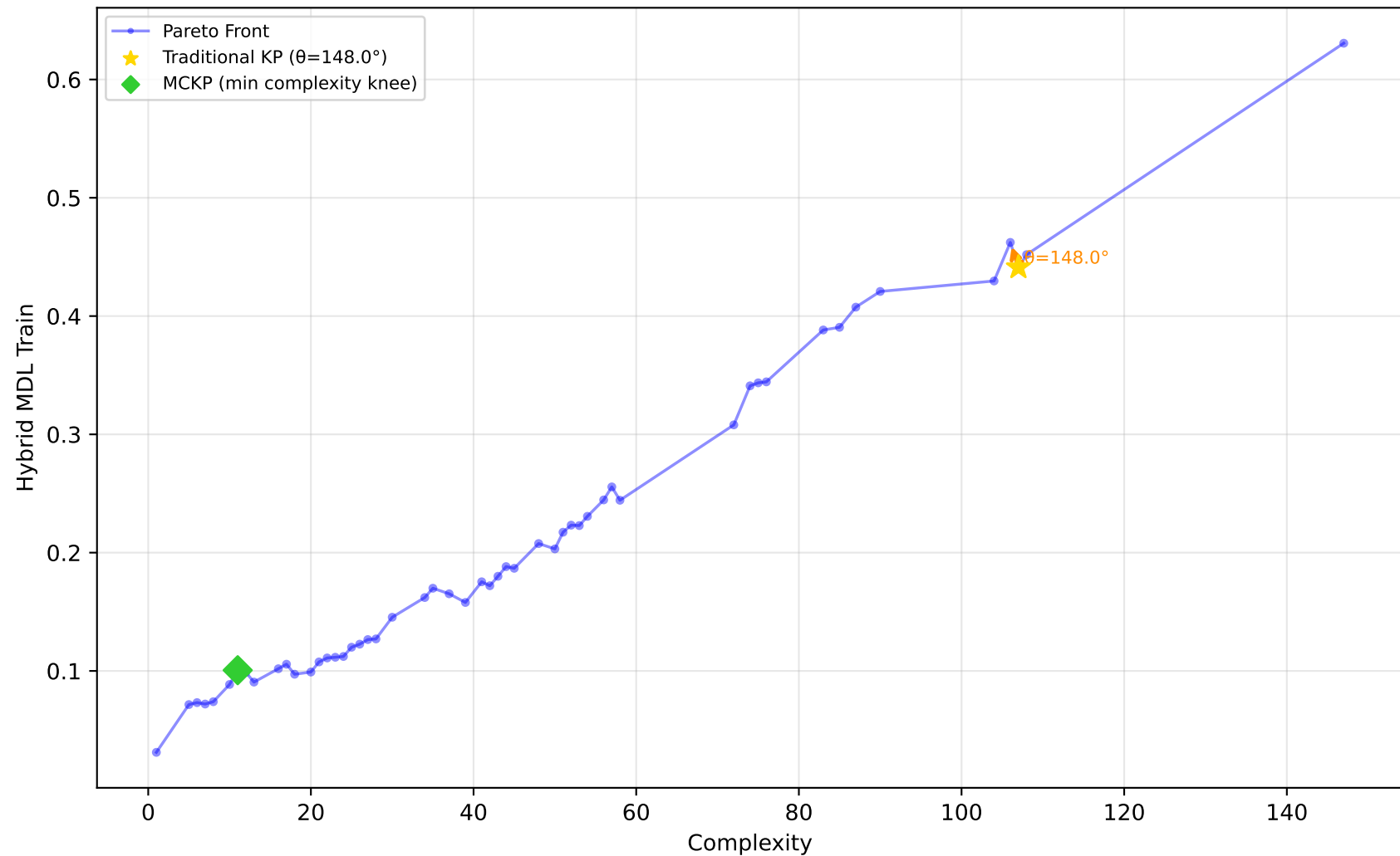
522_pm10 - Run 16 - SVP - Hybrid MDL Train \lambda_1=1.00, \lambda_2=0.00, \lambda_3=0.90 | Difficulty: 1.00 | Method: hmr
