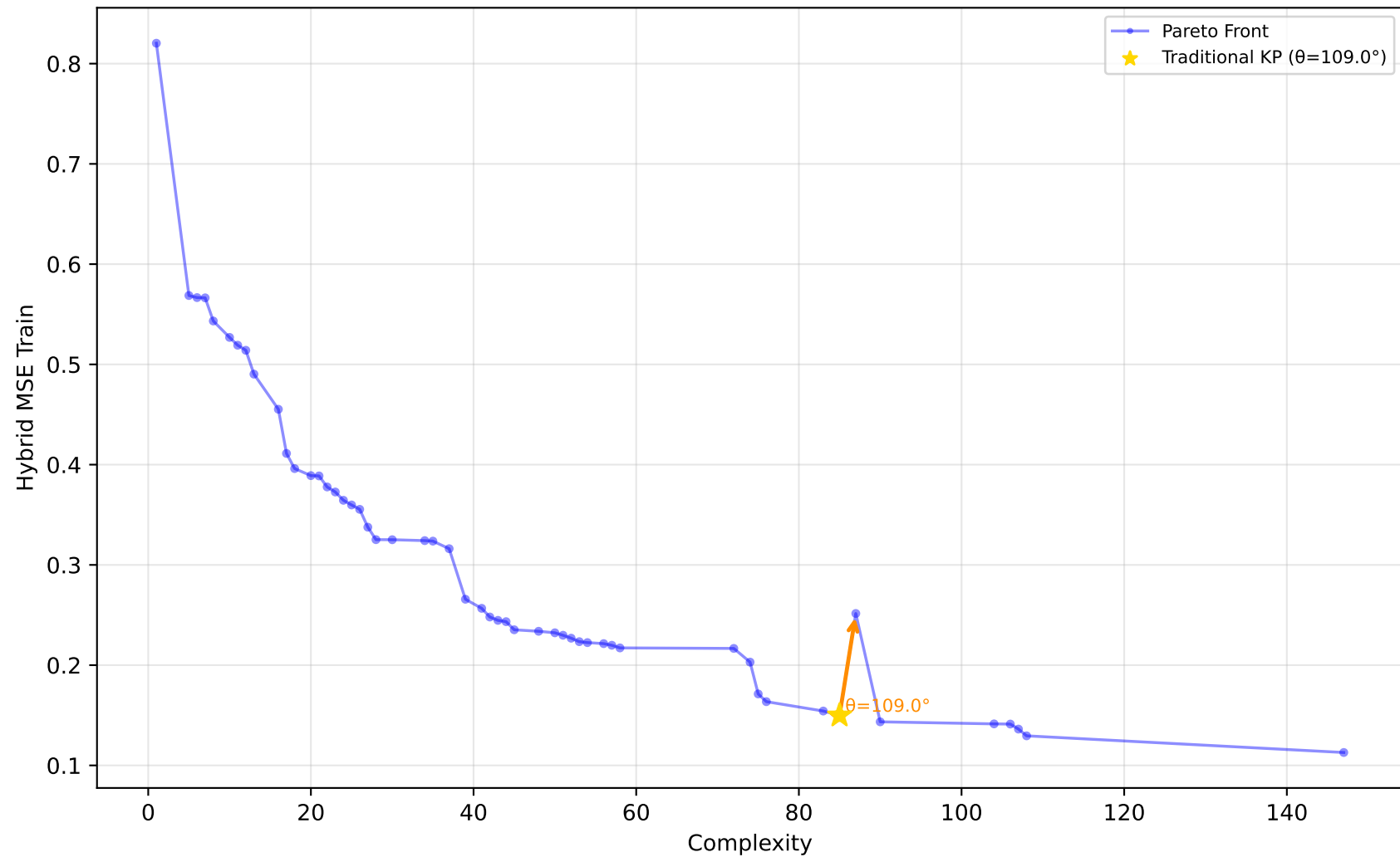
522_pm10 - Run 16 - SVP - Hybrid MSE Train \lambda_1=0.00, \lambda_2=0.10, \lambda_3=0.00 | Difficulty: 1.00 | Method: hmr
