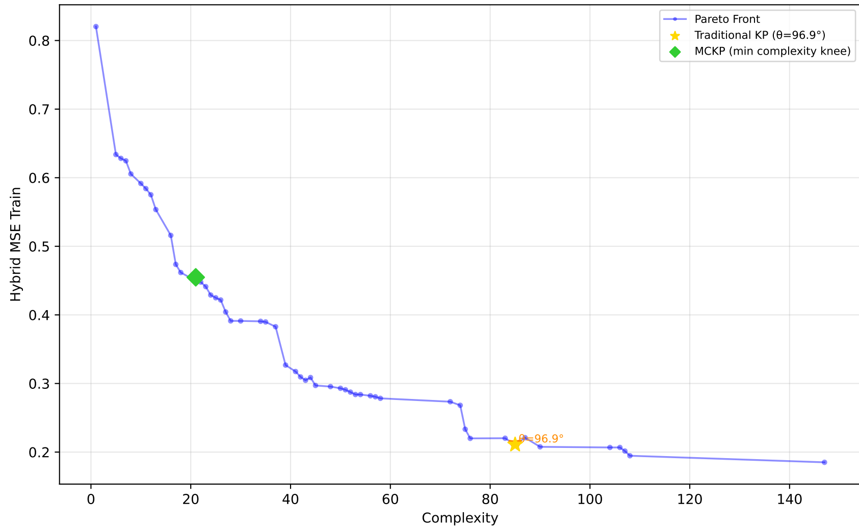
522_pm10 - Run 16 - SVP - Hybrid MSE Train \lambda_1=1.00, \lambda_2=0.00, \lambda_3=0.90 | Difficulty: 1.00 | Method: hmr
