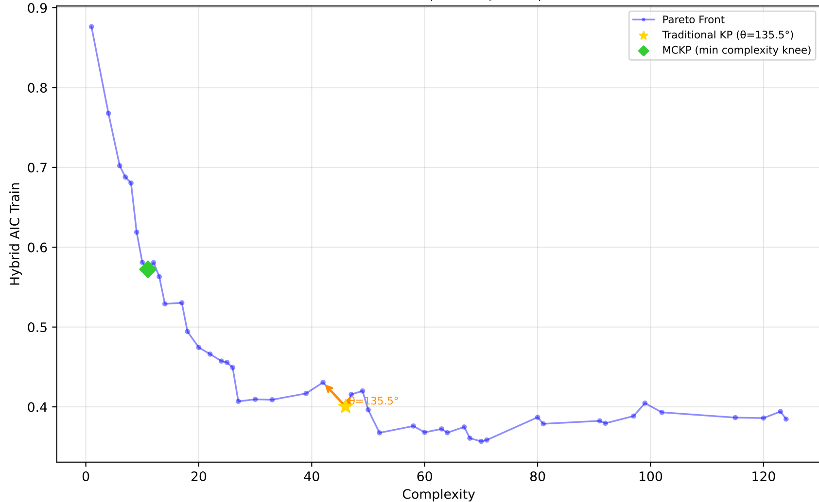
522_pm10 - Run 17 - MVP - Hybrid AIC Train \lambda_1=0.00, \lambda_2=0.90, \lambda_3=0.00 | Difficulty: 0.98 | Method: hmr
