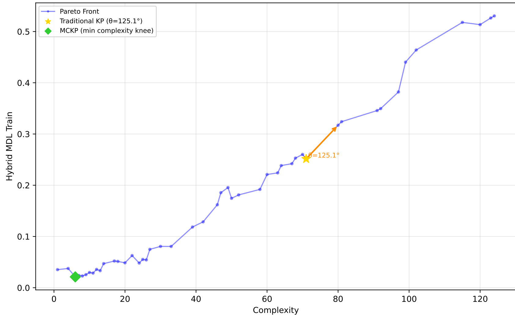
522_pm10 - Run 17 - MVP - Hybrid MDL Train \lambda_1=0.00, \lambda_2=0.90, \lambda_3=0.00 | Difficulty: 0.98 | Method: hmr
