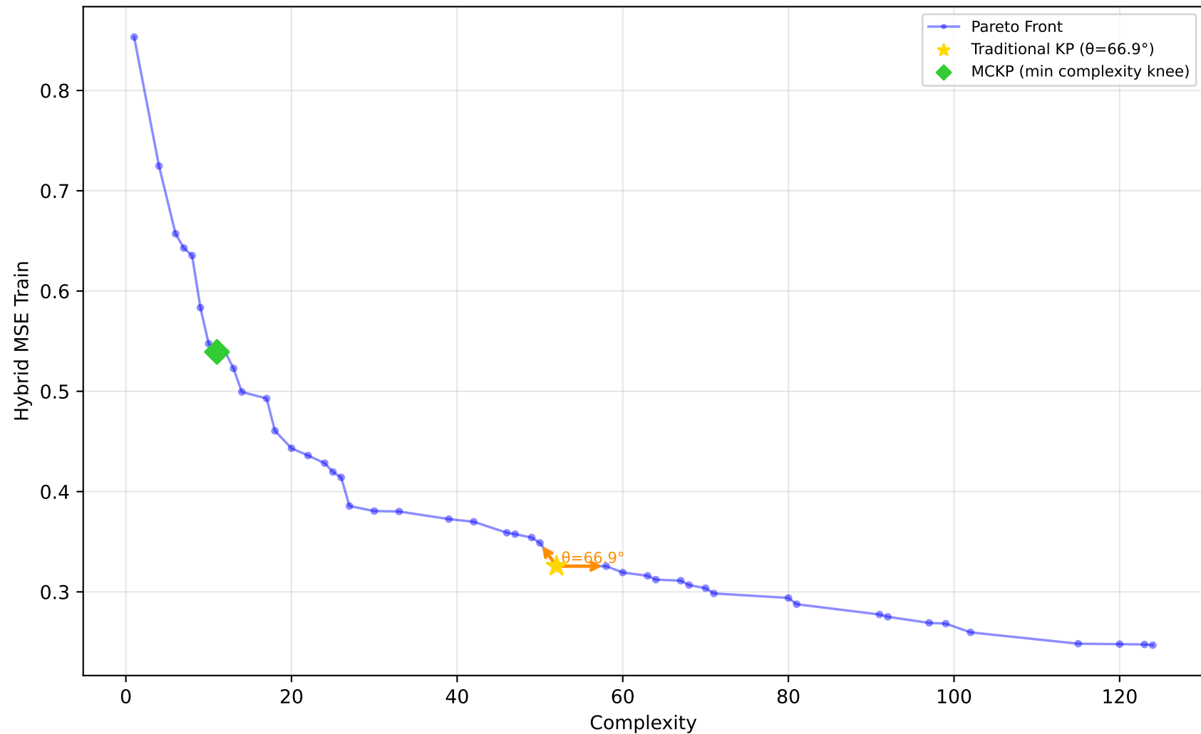
522_pm10 - Run 17 - MVP - Hybrid MSE Train \lambda_1=0.00, \lambda_2=0.90, \lambda_3=0.00 | Difficulty: 0.98 | Method: hmr
