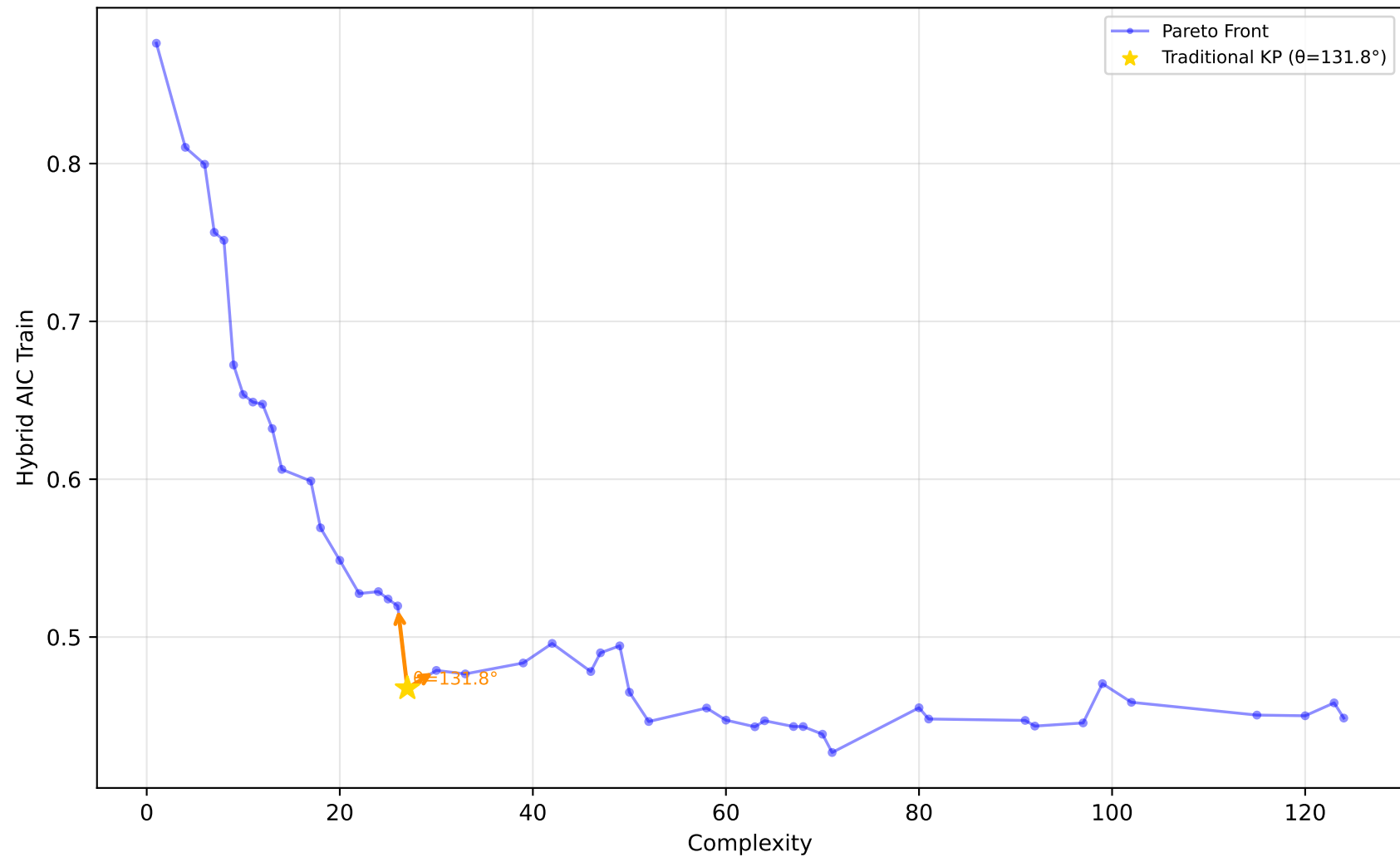
522_pm10 - Run 17 - SVP - Hybrid AIC Train \lambda_1=1.00 , \lambda_2=0.00 , \lambda_3=0.90 | Difficulty: 0.98 | Method: hmr
