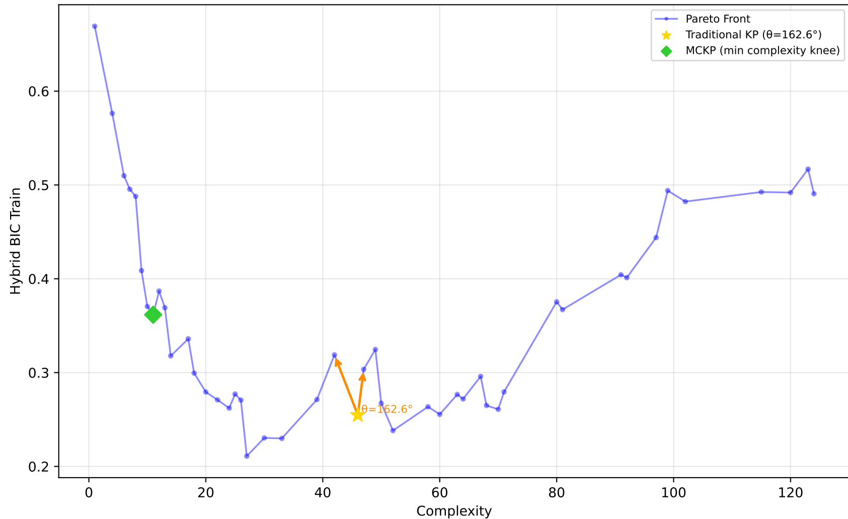
522_pm10 - Run 17 - SVP - Hybrid BIC Train \lambda_1=0.00, \lambda_2=0.10, \lambda_3=0.00 | Difficulty: 0.98 | Method: hmr
