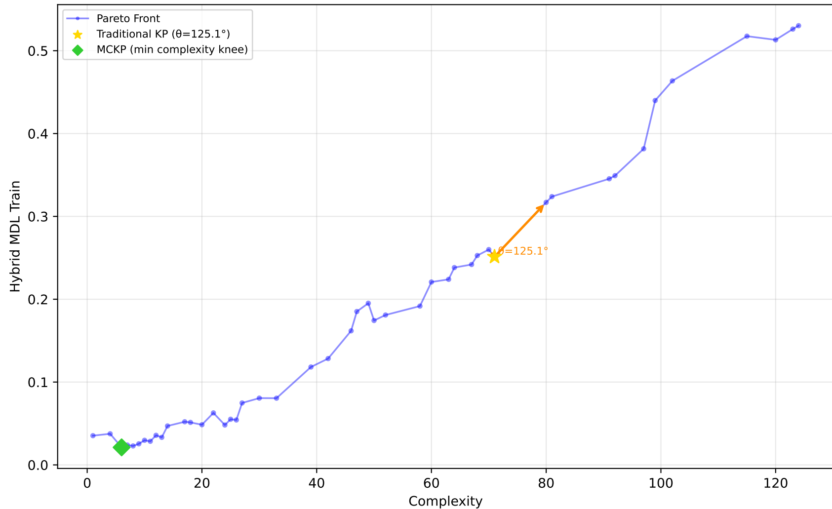
522_pm10 - Run 17 - SVP - Hybrid MDL Train \lambda_1=0.00, \lambda_2=0.10, \lambda_3=0.00 | Difficulty: 0.98 | Method: hmr
