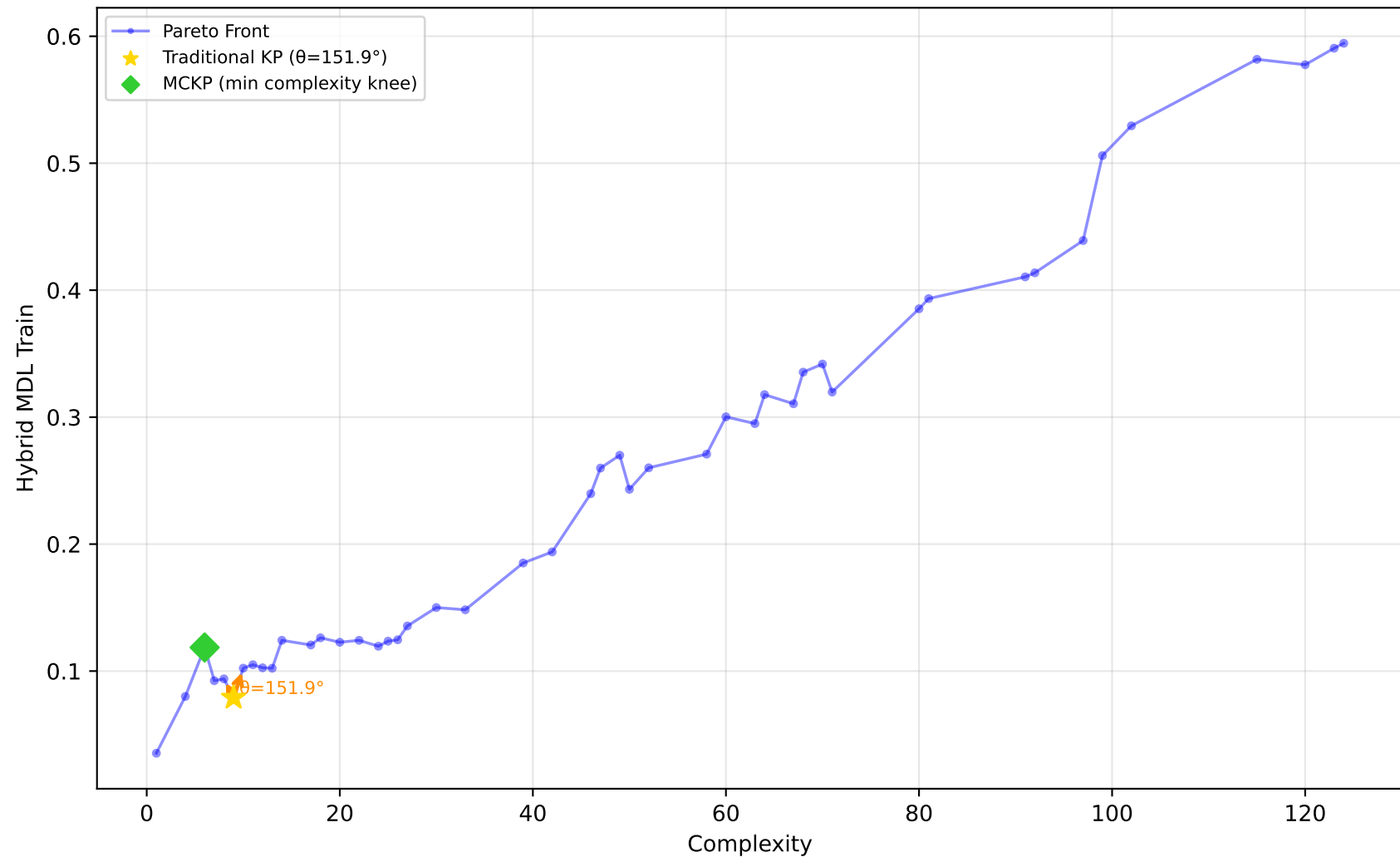
522_pm10 - Run 17 - SVP - Hybrid MDL Train \lambda_1=1.00, \lambda_2=0.00, \lambda_3=0.90 | Difficulty: 0.98 | Method: hmr
