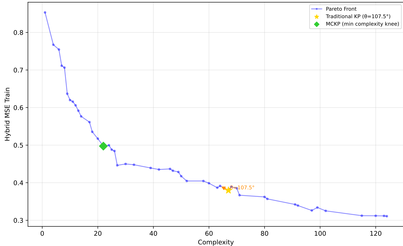
522_pm10 - Run 17 - SVP - Hybrid MSE Train \lambda_1=1.00, \lambda_2=0.00, \lambda_3=0.90 | Difficulty: 0.98 | Method: hmr
