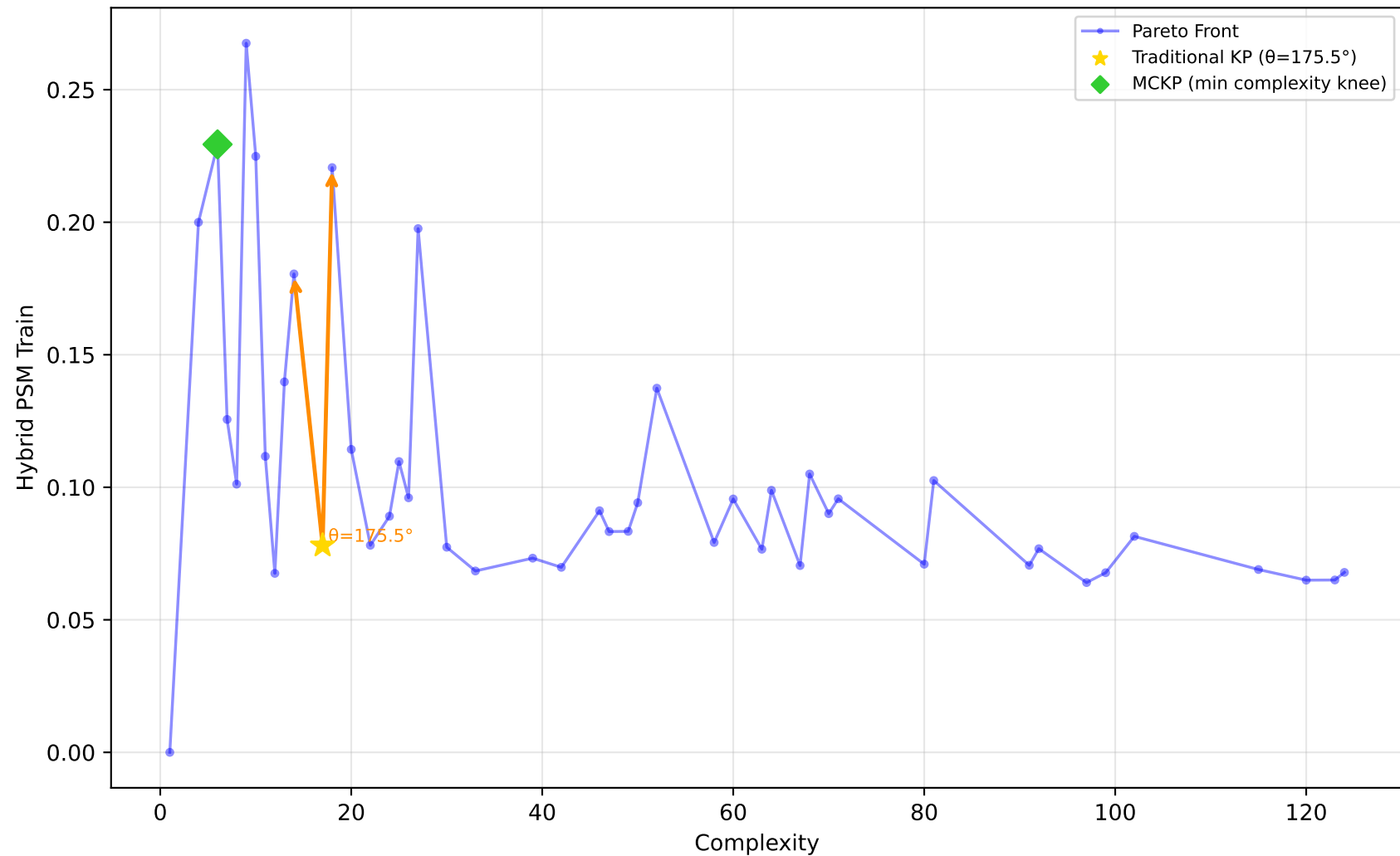
522_pm10 - Run 17 - SVP - Hybrid PSM Train \lambda_1=1.00, \lambda_2=0.00, \lambda_3=0.90 | Difficulty: 0.98 | Method: hmr
