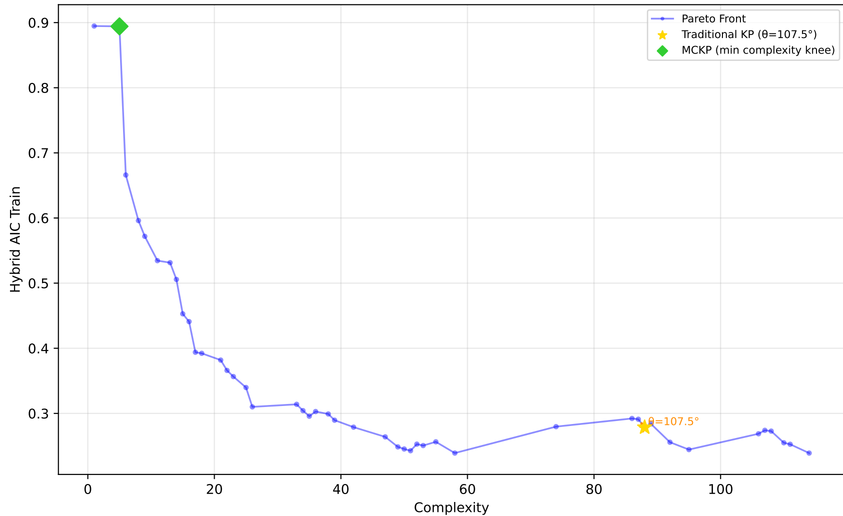
522_pm10 - Run 18 - MVP - Hybrid AIC Train \lambda_1=0.00, \lambda_2=0.90, \lambda_3=0.00 | Difficulty: 1.00 | Method: hmr
