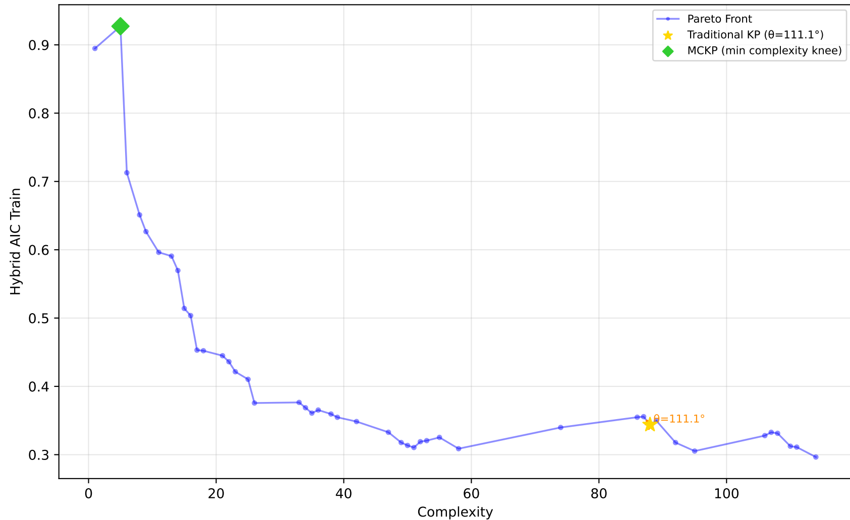
522_pm10 - Run 18 - MVP - Hybrid AIC Train \lambda_1=1.00, \lambda_2=0.00, \lambda_3=0.00 | Difficulty: 1.00 | Method: hmr
