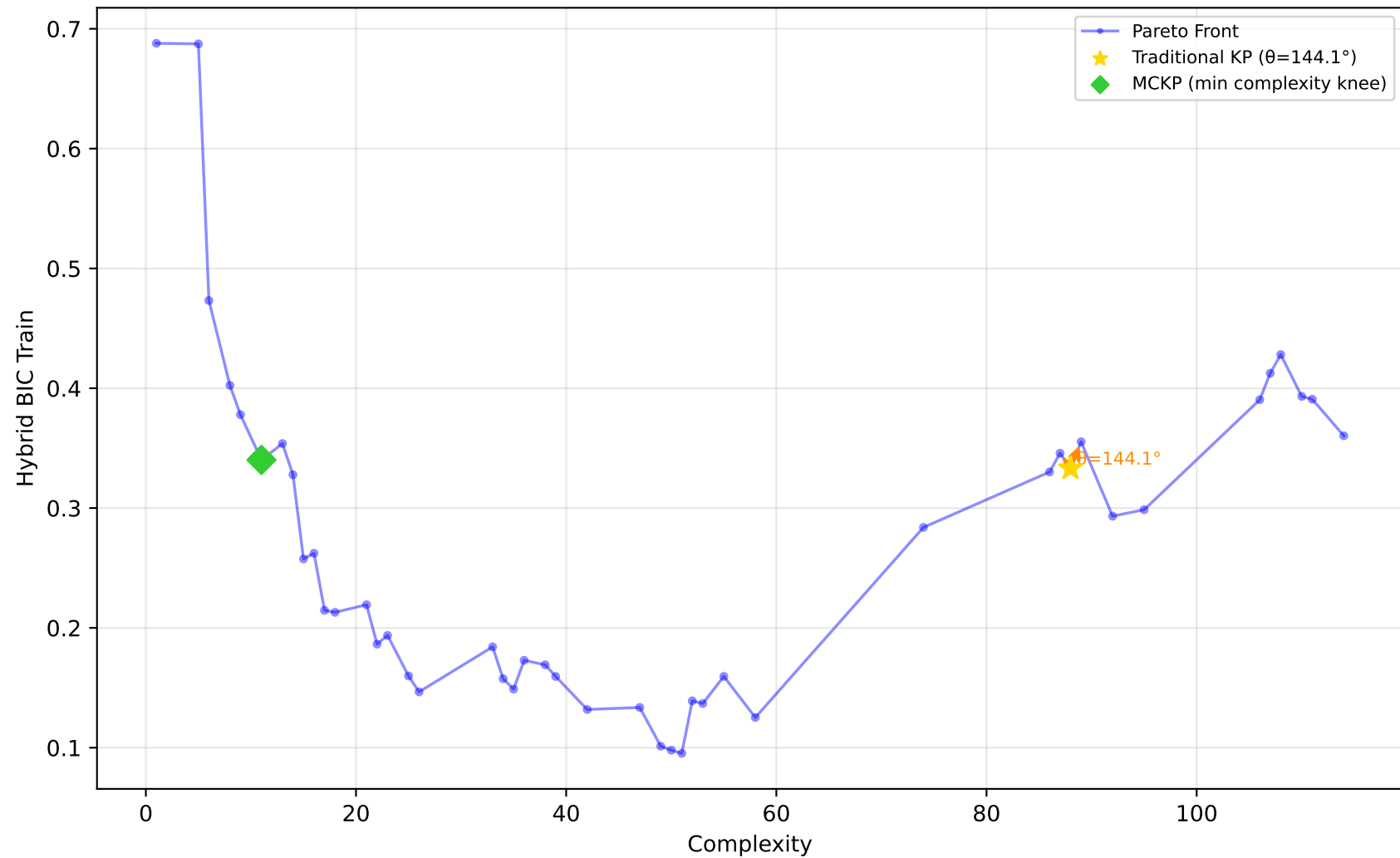
522_pm10 - Run 18 - MVP - Hybrid BIC Train \lambda_1=0.00, \lambda_2=0.90, \lambda_3=0.00 | Difficulty: 1.00 | Method: hmr
