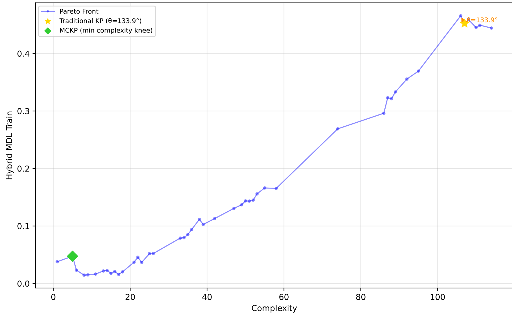
522_pm10 - Run 18 - MVP - Hybrid MDL Train \lambda_1=0.00, \lambda_2=0.90, \lambda_3=0.00 | Difficulty: 1.00 | Method: hmr
