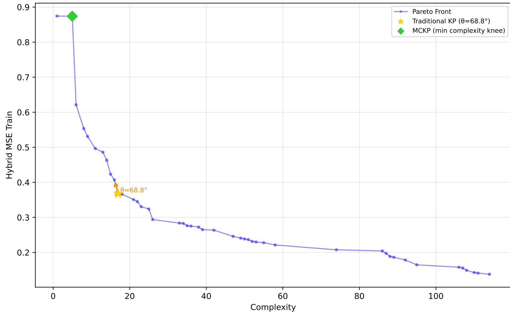
522_pm10 - Run 18 - MVP - Hybrid MSE Train \lambda_1=0.00, \lambda_2=0.90, \lambda_3=0.00 | Difficulty: 1.00 | Method: hmr
