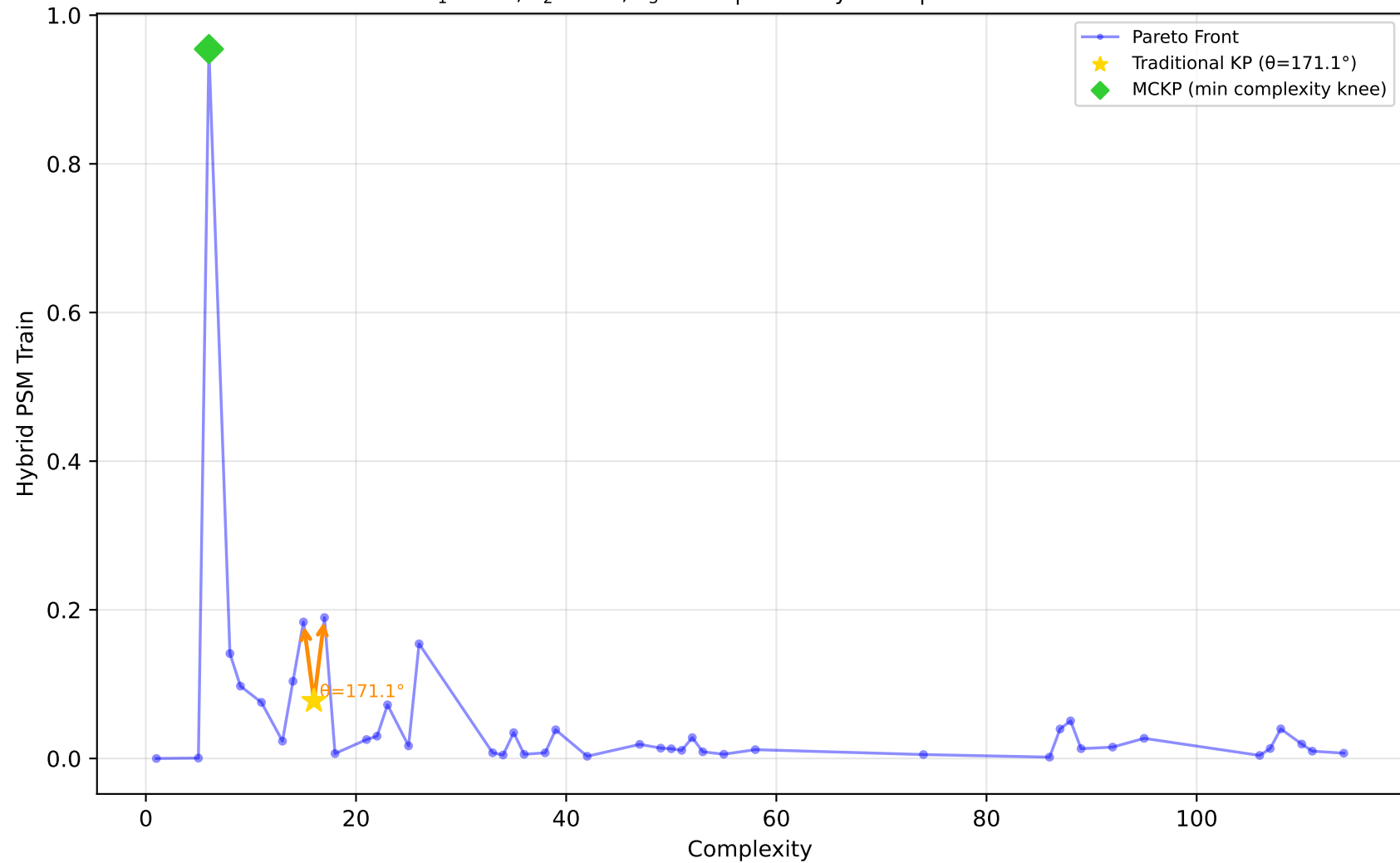
522_pm10 - Run 18 - MVP - Hybrid PSM Train \lambda_1=0.00, \lambda_2=0.90, \lambda_3=0.00 | Difficulty: 1.00 | Method: hmr
