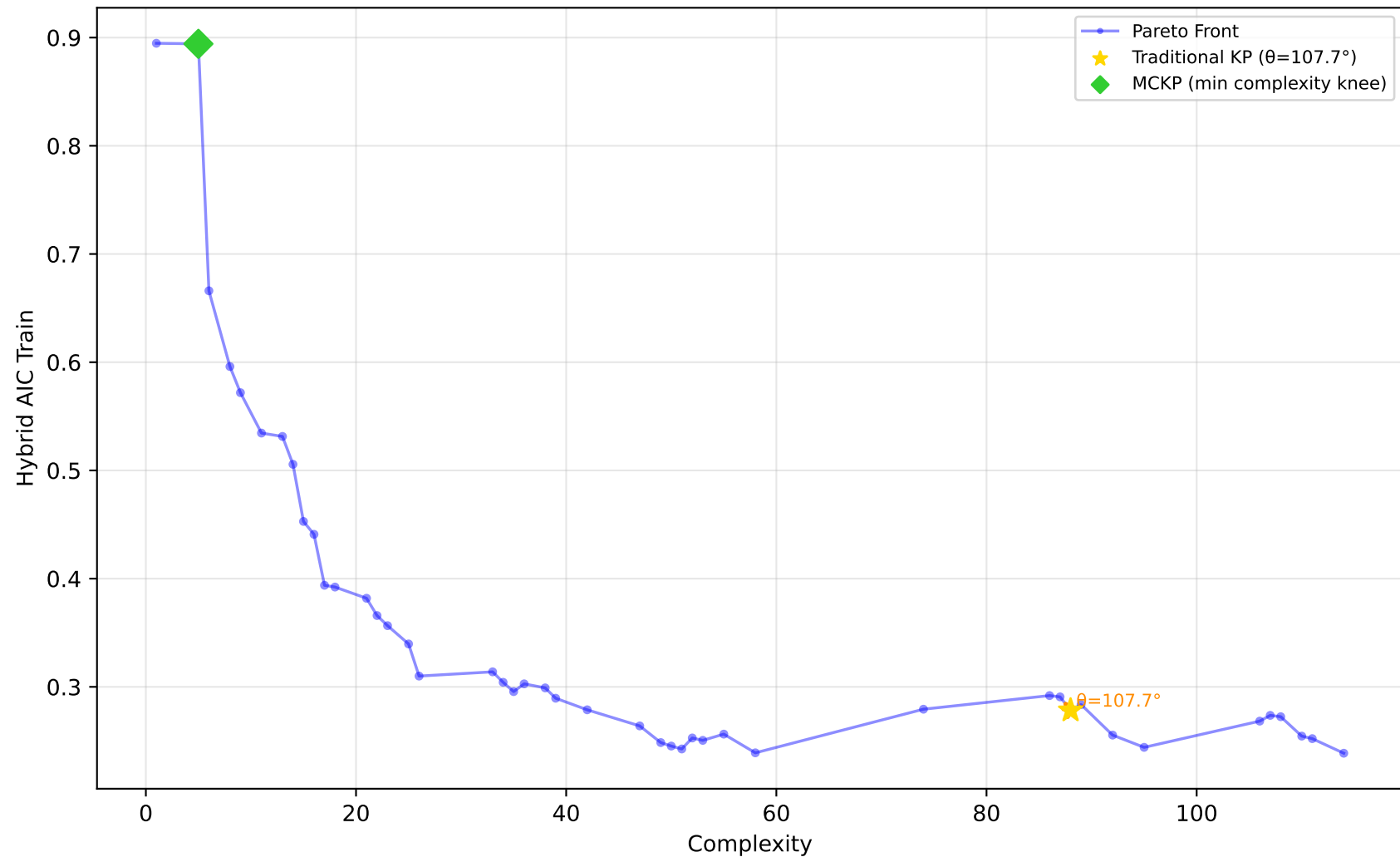
522_pm10 - Run 18 - SVP - Hybrid AIC Train \lambda_1=0.00, \lambda_2=0.10, \lambda_3=0.00 | Difficulty: 1.00 | Method: hmr
