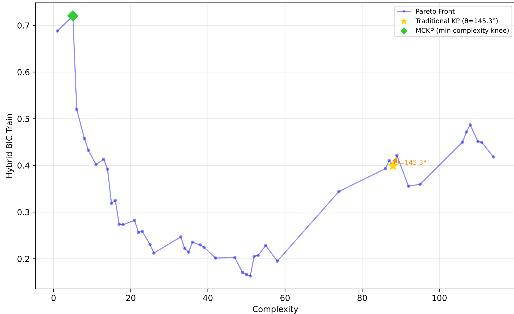
522_pm10 - Run 18 - SVP - Hybrid BIC Train \lambda_1=1.00, \lambda_2=0.00, \lambda_3=0.90 | Difficulty: 1.00 | Method: hmr
