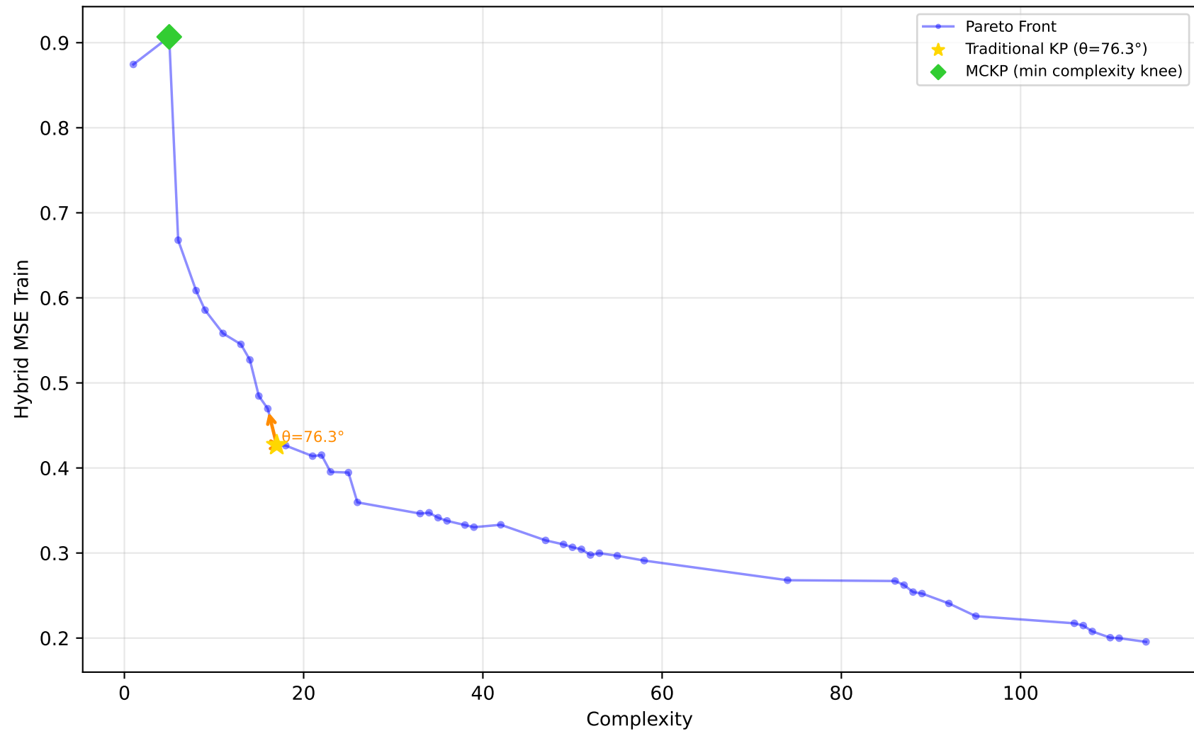
522_pm10 - Run 18 - SVP - Hybrid MSE Train \lambda_1=1.00, \lambda_2=0.00, \lambda_3=0.90 | Difficulty: 1.00 | Method: hmr
