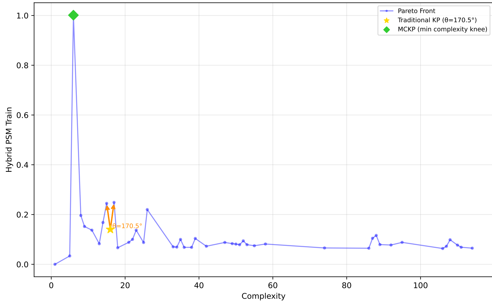
522_pm10 - Run 18 - SVP - Hybrid PSM Train \lambda_1=1.00, \lambda_2=0.00, \lambda_3=0.90 | Difficulty: 1.00 | Method: hmr
