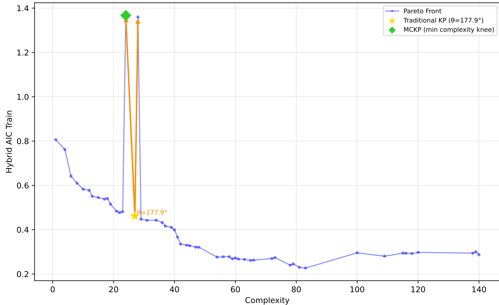
522_pm10 - Run 19 - MVP - Hybrid AIC Train \lambda_1=0.00, \lambda_2=0.90, \lambda_3=0.00 | Difficulty: 1.00 | Method: hmr
