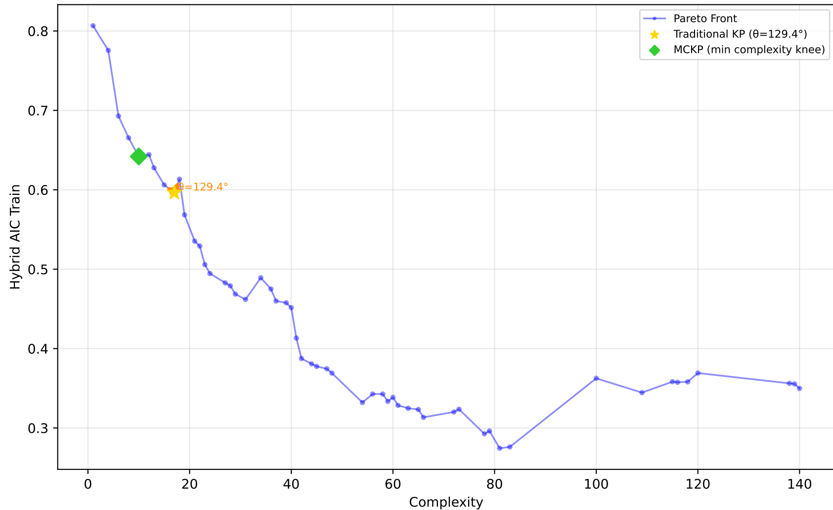
522_pm10 - Run 19 - MVP - Hybrid AIC Train \lambda_1=1.00, \lambda_2=0.00, \lambda_3=0.00 | Difficulty: 1.00 | Method: hmr
