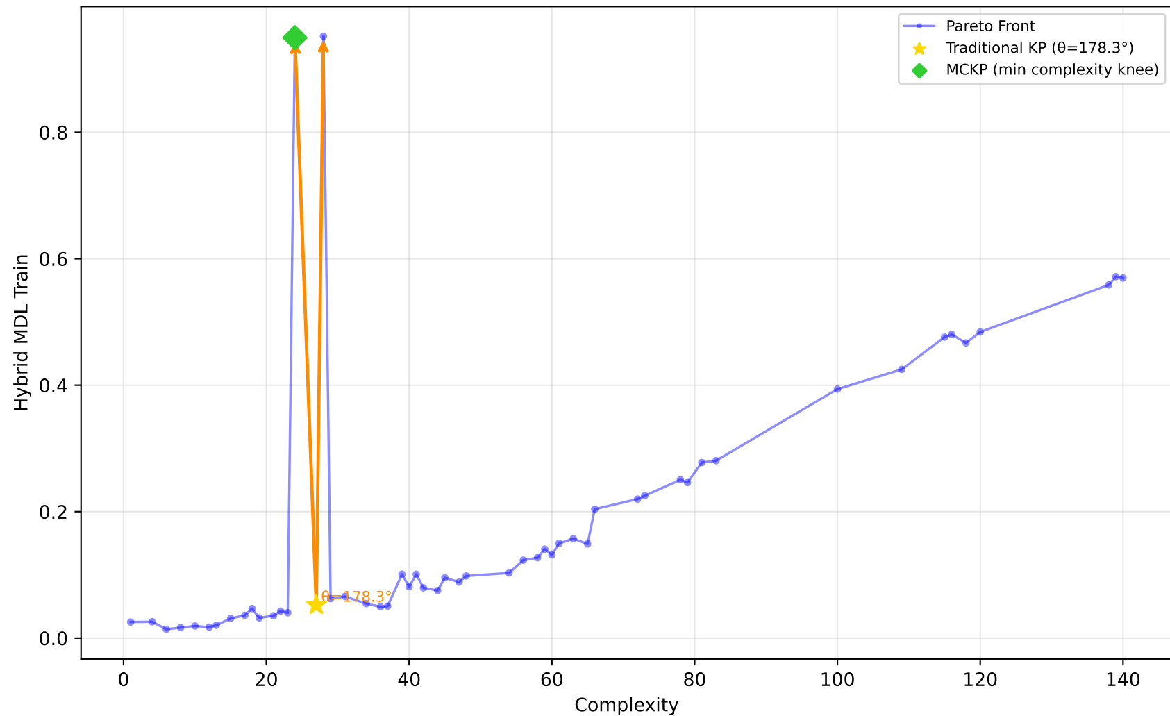
522_pm10 - Run 19 - MVP - Hybrid MDL Train \lambda_1=0.00, \lambda_2=0.90, \lambda_3=0.00 | Difficulty: 1.00 | Method: hmr
