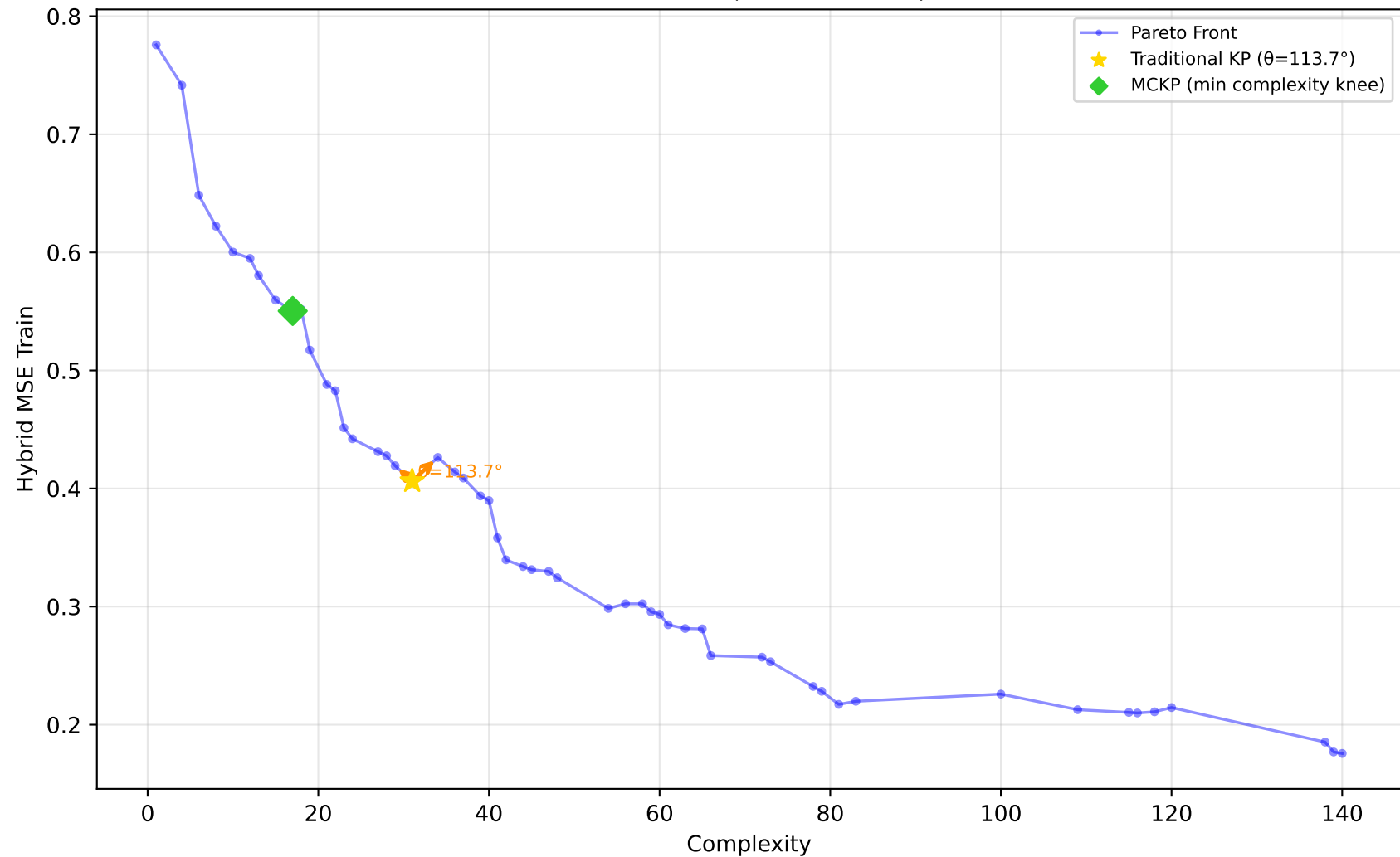
522_pm10 - Run 19 - MVP - Hybrid MSE Train \lambda_1=1.00, \lambda_2=0.00, \lambda_3=0.00 | Difficulty: 1.00 | Method: hmr
