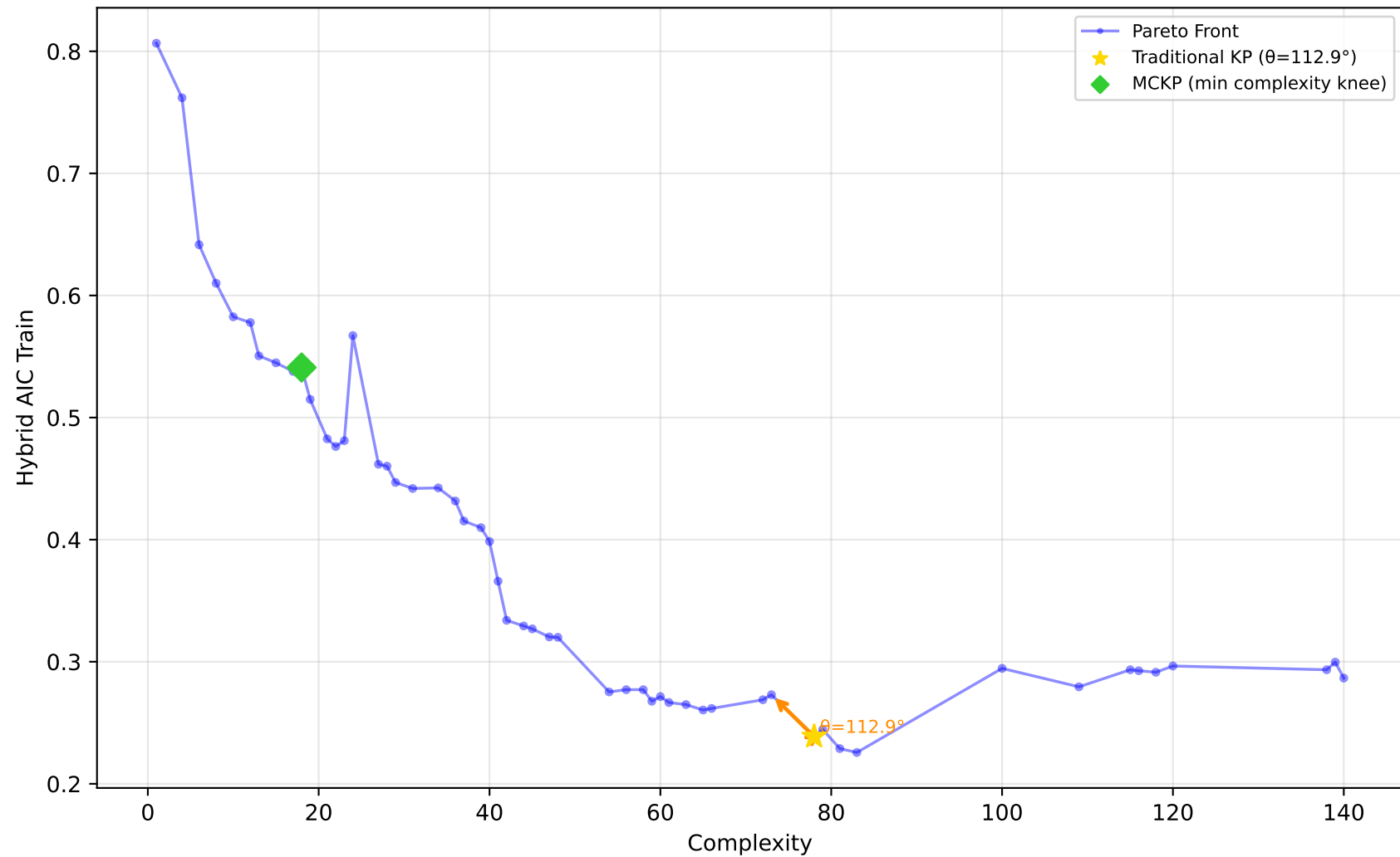
522_pm10 - Run 19 - SVP - Hybrid AIC Train \lambda_1=0.00, \lambda_2=0.10, \lambda_3=0.00 | Difficulty: 1.00 | Method: hmr
