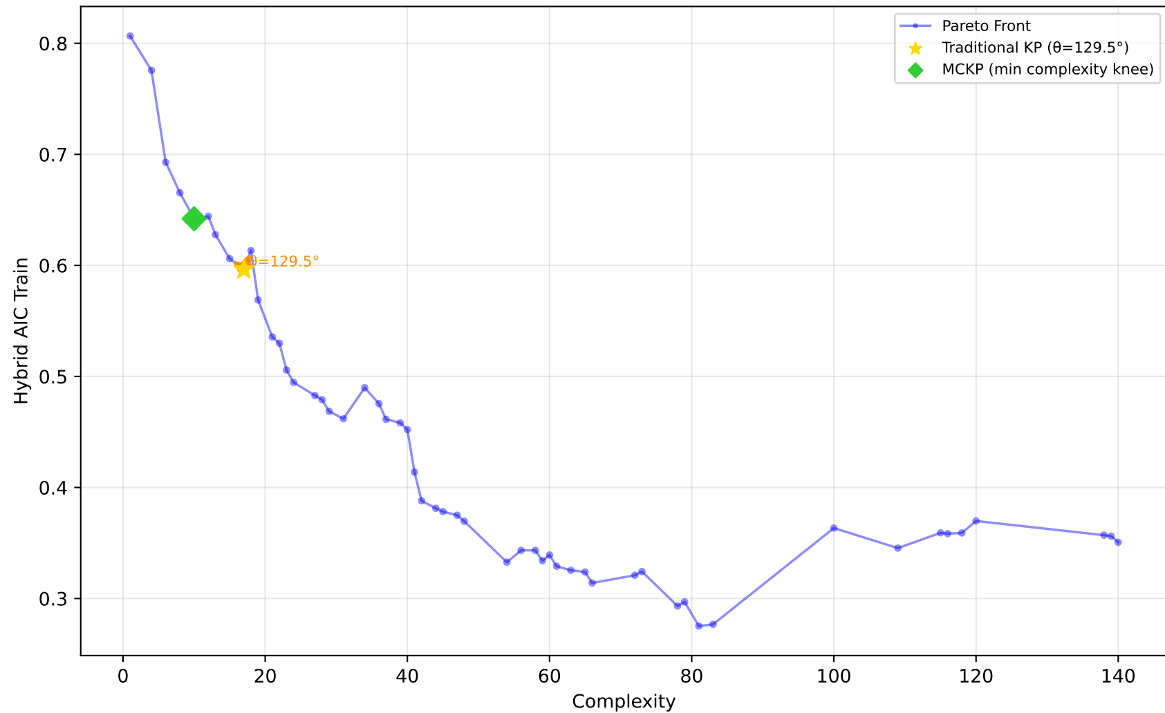
522_pm10 - Run 19 - SVP - Hybrid AIC Train \lambda_1=1.00, \lambda_2=0.00, \lambda_3=0.90 | Difficulty: 1.00 | Method: hmr
