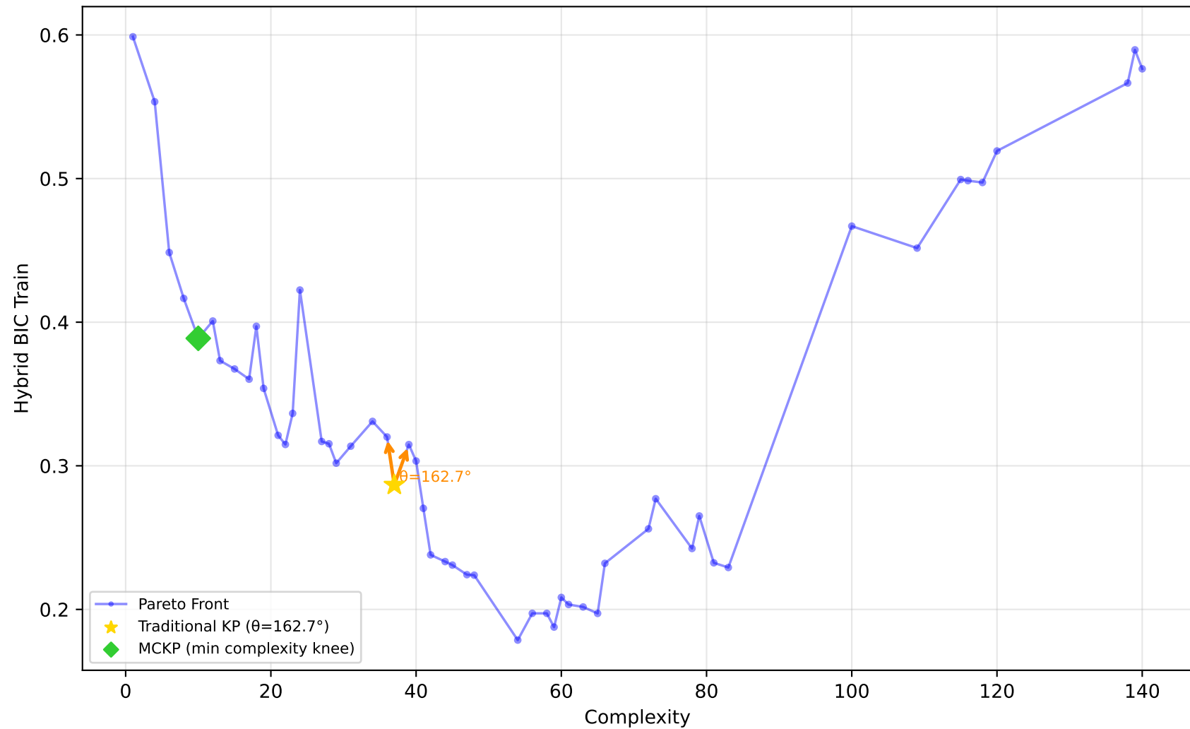
522_pm10 - Run 19 - SVP - Hybrid BIC Train \lambda_1=0.00, \lambda_2=0.10, \lambda_3=0.00 | Difficulty: 1.00 | Method: hmr
