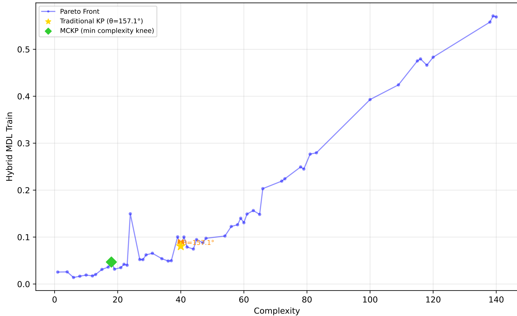
522_pm10 - Run 19 - SVP - Hybrid MDL Train \lambda_1=0.00, \lambda_2=0.10, \lambda_3=0.00 | Difficulty: 1.00 | Method: hmr
