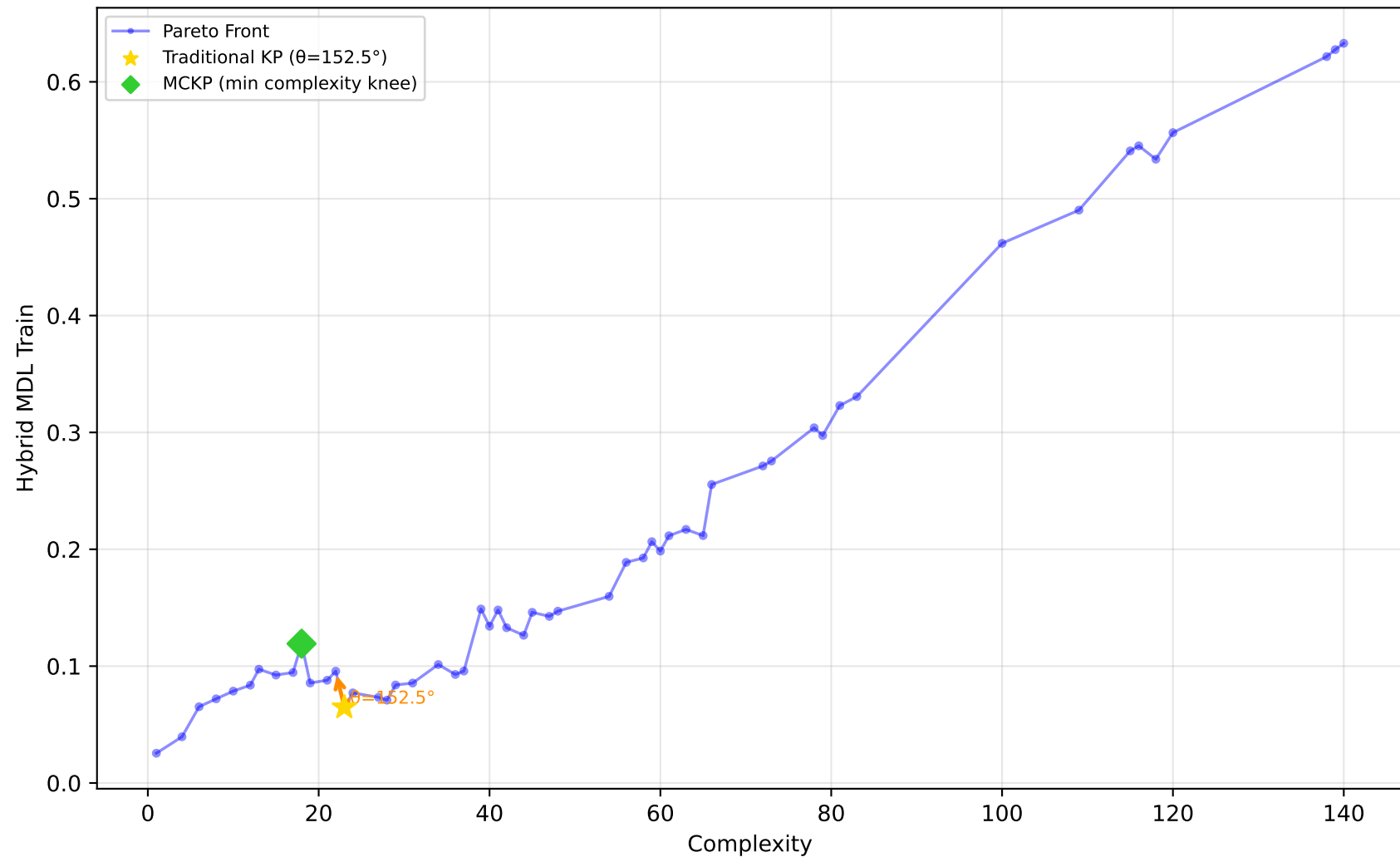
522_pm10 - Run 19 - SVP - Hybrid MDL Train \lambda_1=1.00, \lambda_2=0.00, \lambda_3=0.90 | Difficulty: 1.00 | Method: hmr
