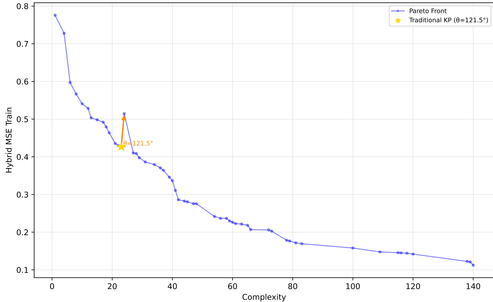
522_pm10 - Run 19 - SVP - Hybrid MSE Train \lambda_1=0.00, \lambda_2=0.10, \lambda_3=0.00 | Difficulty: 1.00 | Method: hmr
