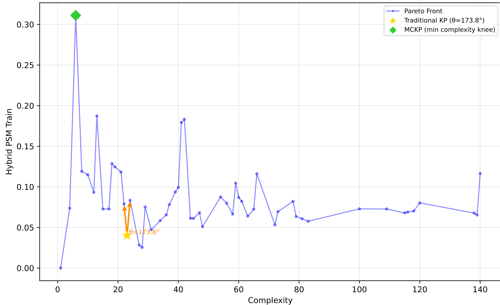
522_pm10 - Run 19 - SVP - Hybrid PSM Train \lambda_1=1.00, \lambda_2=0.00, \lambda_3=0.90 | Difficulty: 1.00 | Method: hmr
